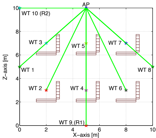
Fig. 11. Office scenario with two relay WTs.
