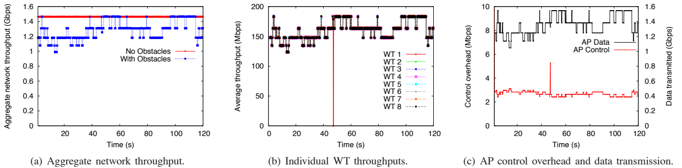
Fig. 9. Protocol performance: office scenario with single relay.
