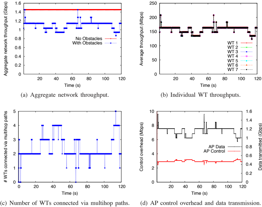
Fig. 8. Protocol performance: living room scenario.
