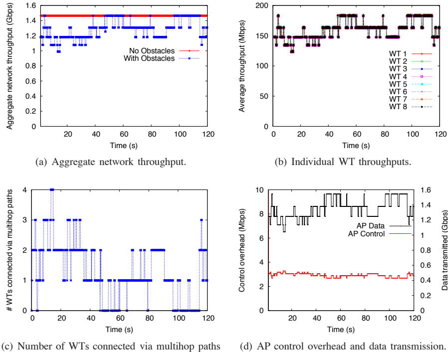
Fig. 10. Protocol performance: office scenario with two relays.
