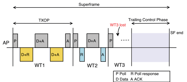
Fig. 6. An example MAC message sequence over a superframe.
