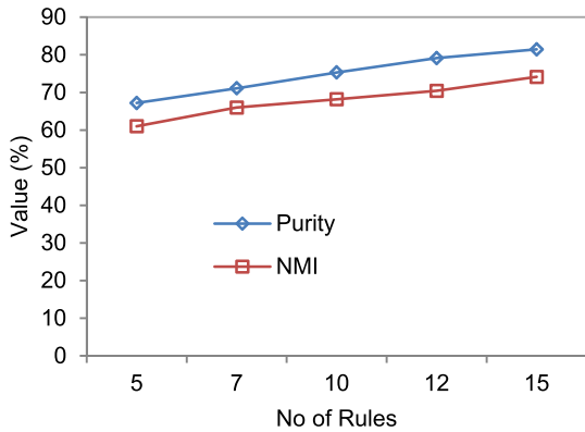
FIGURE 16. Purity and NMI for heart data.
