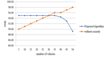
Figure 5. PDR with increasing vehicles
