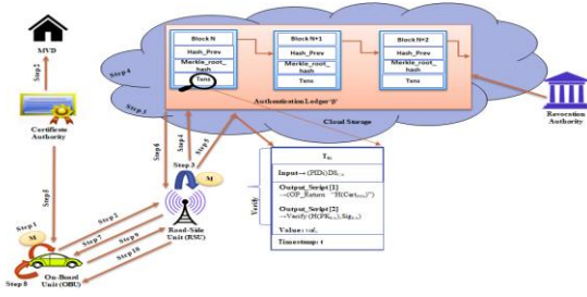
Figure 1. Mutual Authentication of OBU-RSU
