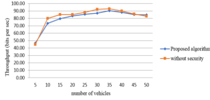
Figure 4. Throughput with increasing vehicles
