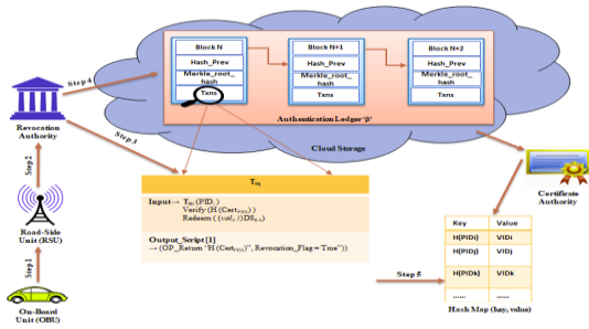
Figure 2. Revocation of malicious vehicle
