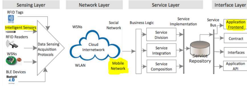
Fig. 1. An architecture of an IIoT platform [4]
