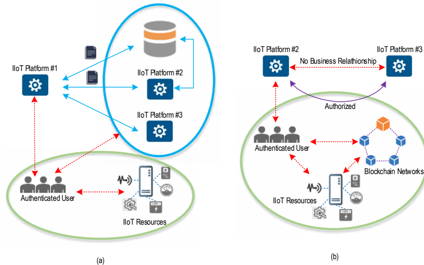
Fig. 5. IIoT architecture to convert real-time data into business insights (Interoperability)
