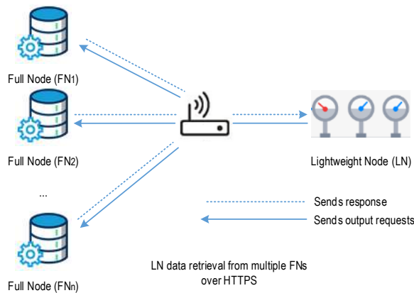
Fig. 3. LN data retrieval from multiple FNs
