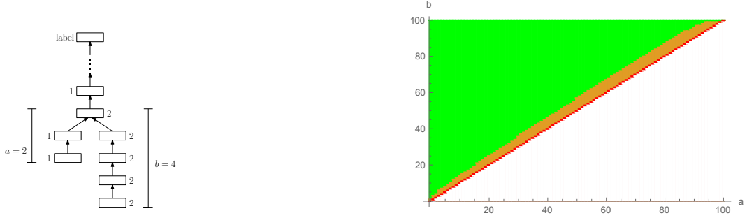
Figure 1: On the left, a typical state (tree). On the right, the set of states form the optimal strategy for the truncated game at d = 100 . The upper-left green part is the set C of capitulating states, the diagonal red line is the set W of winning states, and the orange part the set M of mining states.
