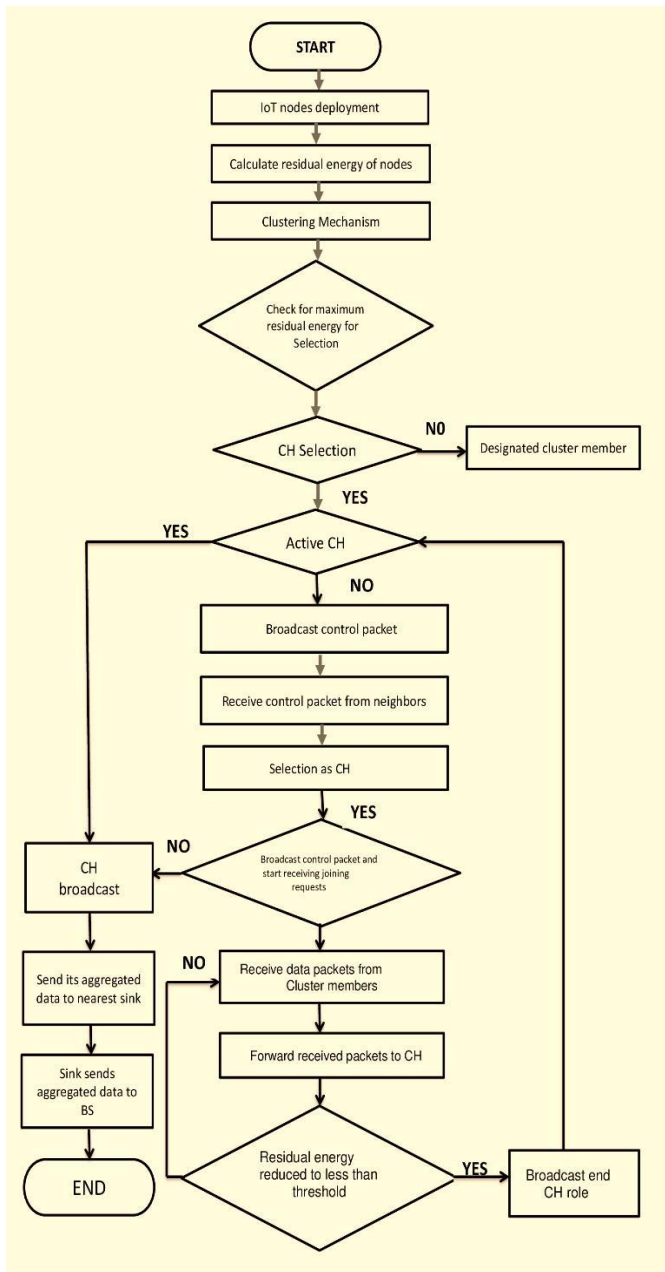
Fig 9. Flowchart for IoT with Blockchain.
