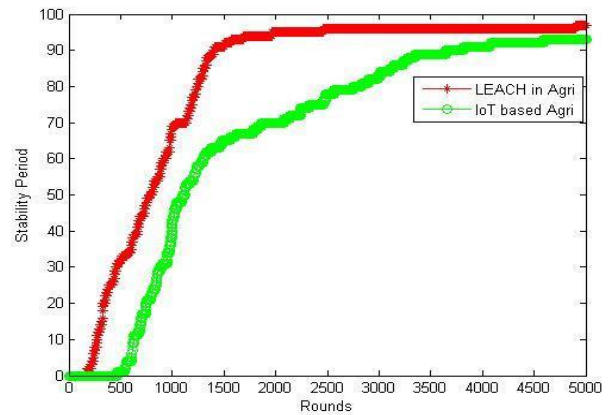
Fig 11. Stability period of LEACH Vs IoT.
