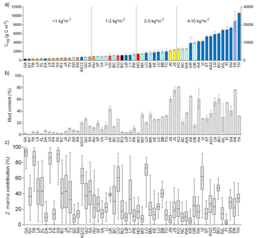
Figure 2. (a) C_{org} stocks ( \text{g C m}^{-2} \pm \text{SE} ) in the top 25 cm of sediment at all sites. Note that value at site TH corresponds to right y axis. (b) Sediment mud content ( \% \pm \text{SE} ) and (c) the relative contribution of Z. marina tissues to the \delta^{13}\text{C} of the sediment surface layer (0–5 cm) at the sites. Box plots represents first and third quartiles and are shown with medians (horizontal line), means (+). The whiskers represent the 2.5–97.5th percentiles. Z. marina contribution was calculated from a pooled \delta^{13}\text{C} value of aboveground and belowground tissue. Sites are ordered according to the magnitude of C_{org} stocks (from lowest to highest). In Figure 2a, the sites are colored according to the study region: Black = Black Sea; brown = Baltic Sea; dark blue = Kattegat-Skagerrak; turquoise = Eastern Pacific; light blue = Western Atlantic; red = eastern Atlantic; yellow = Western Pacific; purple = Mediterranean Sea. For site names, see Table S1.
