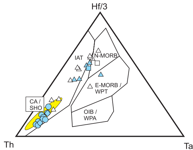
Fig. 7. Hf/3-Th-Ta discriminant diagram (Wood 1980) for the blueschists with volcanic starting rocks from the Cretaceous conglomerates of the Klappe Unit (filled symbols) compared to their analogues from the Bôrka Nappe of the Meliatic Unit (opens symbols). Shaded field represents positions of LP/LT volcanic rocks from conglomerates of the Klappe Unit. Explanations: triangles – basalts, diamonds – andesites, circles – dacites and rhyolites, squares – amphibolites with blueschist facies overprint, CA/SHO – calc-alkaline/shoshonite volcanics, IAT – island arc tholeiites, OIB/WPA – oceanic island basalts/within-plate alkali basalts, E-MORB/WPT – enriched mid-ocean ridge basalts/within-plate tholeiites, N-MORB – normal mid-ocean ridge basalts
