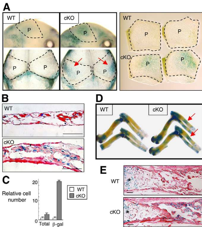
Fig. 4. Upregulation of canonical Wnt signaling in Bmpr1a cKO mice. (A) Canonical Wnt signaling assessed by TOPGAL mice using E17.5 calvariae (upper panel, lateral view; lower panel, top view). Two independent parietal bones from two littermates in each group after dissection are shown in the right-hand panel. Red arrow indicates enhanced Wnt signaling. Broken line, areas of parietal bones (P). (B) Histological analysis assessed by TOPGAL mice using E17.5 calvariae. Scale bars: 50 \mu m. (C) Relative cell number of DAPI and \beta -gal positive cells. Cells were counted in 50 fields of E17.5 calvariae from cKO ( n=4 ) and wild type ( n=4 ). Total cell number was obtained by counting DAPI-positive nuclei in bone. Cell number of wild type is set as 1.0. There were 2.3 times more total cells in cKO calvariae in a given section than in wild type owing to the thicker tissues, but the number of \beta -gal-positive cells was 19.7 times greater, resulting in an 8.5-fold increase in the proportion of \beta -gal positive cells in cKO mice. (D) Canonical Wnt signaling assessed by TOPGAL mice using humerus, ulna and radius at E17.5. Red arrow indicates enhanced Wnt signaling. (E) Histological analysis assessed by TOPGAL mice using radius at E17.5. Asterisks, growth plates. Scale bars: 100 \mu m.
