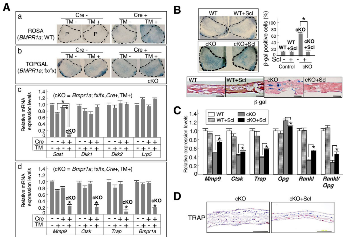
Fig. 6. Suppressed expression of sclerostin by loss of BMP signaling ex vivo. (A) Newborn mouse calvariae were cultured for 5 days treated with 4OH-TM (100 ng/ml). (a) Confirmation of Cre activity in the calvariae from CreER:R26R mice assessed by \beta -gal staining. (b) Upregulation of canonical Wnt signaling in the calvariae from CreER:Bmpr1afx/fx:TOPGAL mice assessed by \beta -gal staining. Broken lines, areas of parietal bones (P). (c) Expression of Wnt inhibitors Sost , Dkk1 , Dkk2 and Lrp5 assessed by QRT-PCR. (d) Expressions of bone resorption markers Mmp9 , Ctsk , TRAP and Bmpr1a . Values are expressed relative to those of wild type ( Cre - , TM - ). (B) Sclerostin treatment of wild-type ( WT+Scl ) and cKO ( cKO+Scl ) calvariae ex vivo. The ratio of \beta -gal to DAPI-positive cells was evaluated from 50 fields in frontal sections ( n=3 , in each condition). Broken line, parietal bones. Scale bars: 50 \mu m. (C) Expression of bone resorption markers Rankl and Opg , and relative ratio of Rankl to Opg using wild-type and cKO calvariae in sclerostin treated versus untreated groups. Values are expressed relative to those of wild type without sclerostin treatment. (D) TRAP staining of cKO calvariae treated with sclerostin and non-treated ex vivo. Values in A-C represent mean \pm s.d. from three independent experiments. Student's t -test; * P < 0.05 .
