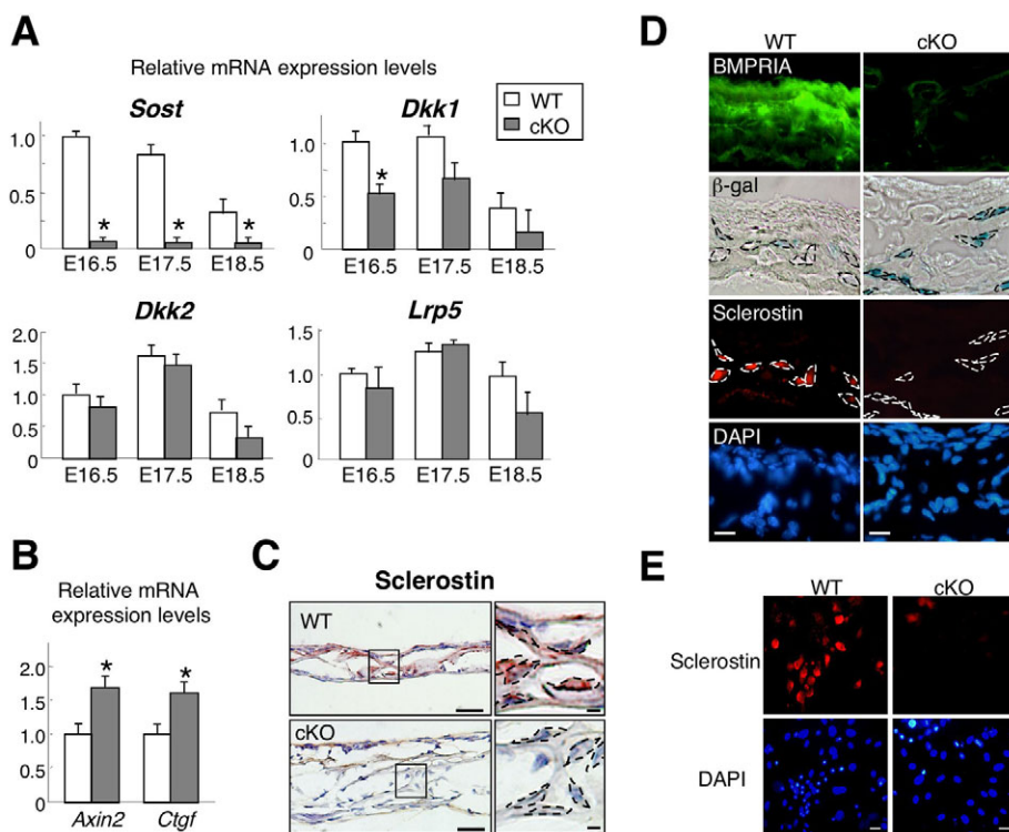
Fig. 5. Inhibition of canonical Wnt signaling by sclerostin in Bmpr1a cKO mice. (A) QRT-PCR analysis for Sost , Dkk1 , Dkk2 and Lrp5 using calvariae at E16.5, E17.5 and E18.5. Values are expressed relative to wild type at E16.5. Student's t -test; * P <0.05. (B) QRT-PCR analysis for Wnt target gene Axin2 and Ctgf using E18.5 calvariae. Expression levels of Axin2 and Ctgf were significantly increased in cKO calvariae. Student's t -test; * P <0.05. (C) Immunohistochemical staining of sclerostin (brown) counterstained with Hematoxylin (blue) using E17.5 calvariae. Broken line, osteoblasts. Scale bars: 50 \mu m, left panel; 10 \mu m, right panel. (D) Detection of BMPR1A (green), canonical Wnt signaling (blue) and sclerostin (red) using E17.5 calvariae. Canonical Wnt signaling was assessed by \beta -gal staining using TOPGAL mice. Nuclei were stained with DAPI (blue). Broken line, osteoblasts. Scale bars: 20 \mu m. (E) Immunohistochemical staining for sclerostin (red) in primary osteoblasts from Bmpr1a cKO and wild-type control. Nuclei were stained with DAPI (blue). Scale bars: 20 \mu m.
