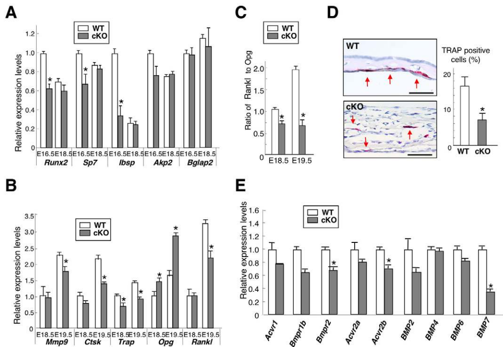
Fig. 3. Alteration of bone formation and resorption in Bmpr1a cKO mice. (A) QRT-PCR for bone formation markers ( Runx2 , Sp7 , Ibsp , Akp2 and Bglap2 ) using E16.5 and E18.5 calvariae. Values are expressed relative to wild type at E16.5. (B) QRT-PCR for bone resorption markers expressed by osteoclasts ( Mmp9 , Ctsk and Trap ), and Rankl and Opg expressed by osteoblasts using E18.5 and E19.5 calvariae. Values are expressed relative to wild type at E18.5. (C) Relative ratio of Rankl to Opg expression levels calculated from Fig. 3B. Values are expressed relative to wild type at E18.5. (D) Evaluation of osteoclast activity by TRAP staining using E18.5 calvariae. The positive cells localized randomly in cKO calvariae compared with wild type (left two panels, red arrows). The percent of TRAP-positive cells per total cells in bone area detected by DAPI was significantly reduced in cKO calvariae (wild type, 13.9%; cKO, 6.4%, right panel). Scale bars: 50 \mu m. (E) QRT-PCR for BMP type I receptors ( Bmpr1b , Acvr1 ), type II receptors ( Bmpr2 , Acvr2a and Acvr2b ) and potential ligands for these receptors ( Bmp2 , Bmp4 , Bmp6 and Bmp7 ) using E18.5 calvariae. Values in A-E represent mean \pm s.d. from a minimum of three independent experiments using wild-type and cKO bones. Student's t-test; * P <0.05.
