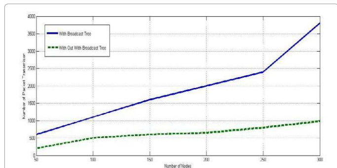
Figure 12: Number of transmission required to broadcast a packet with broadcast tree and without broadcast tree.
