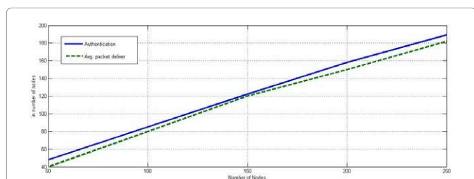
Figure 13: Number of authenticated node and avg. number of node that received the broadcast packet.
