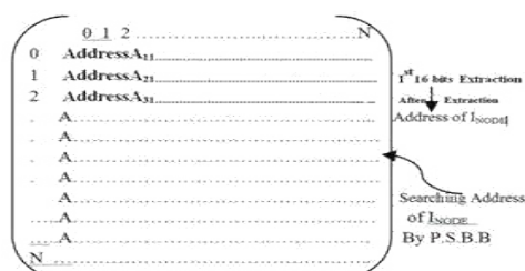
Figure 8: Address Table of I_{Node} holding address of other I_{nodes} .
