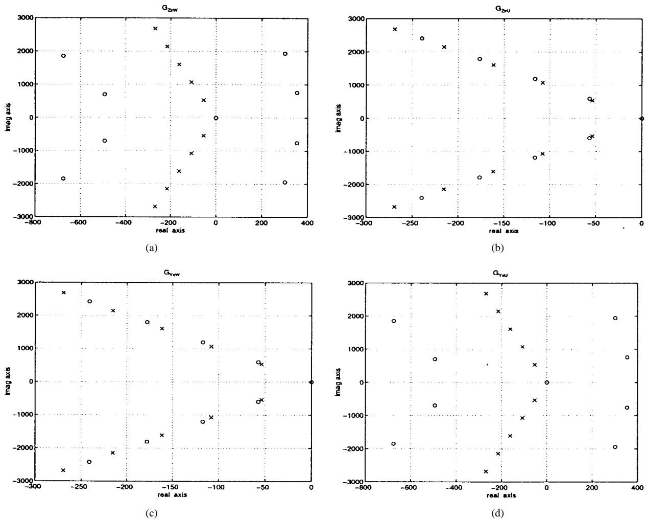
Fig. 4. Pole-zero plots of the transfer functions (a) G_{z_x w}(s) , (b) G_{z_x u}(s) , (c) G_{y_x w}(s) , and (d) G_{y_x u}(s) with noncollocated measurement and performance and with noncollocated control and disturbance show that G_{z_x u}(s) and G_{y_x w}(s) satisfy pole-zero interlacing and thus are minimum phase.
