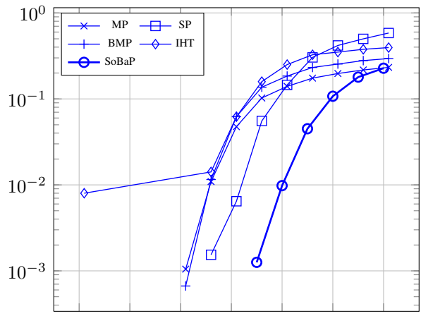
(b) Probability of missed detection
