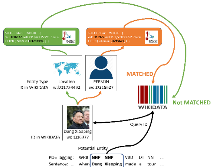
Figure 9: Illustration of matching entities from Wikidata
