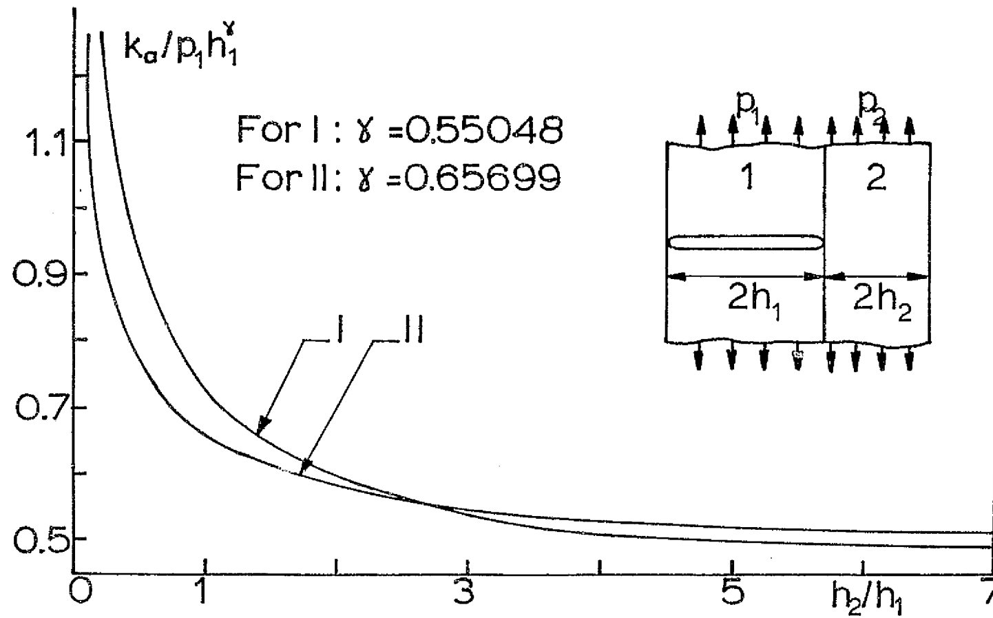
Figure 9 The stress intensity factor k(h_1)=k_a for broken laminates 1 in material combinations I and II
