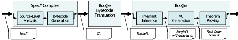
Fig. 0. The Boogie pipeline.
