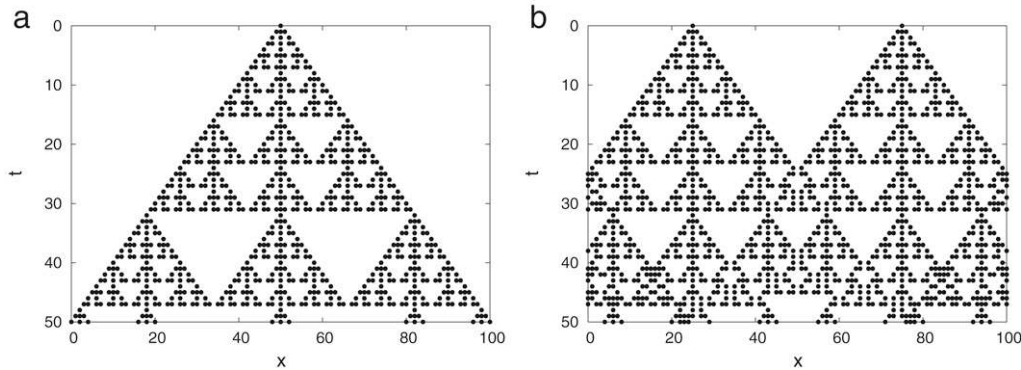
Fig. 13. Solutions of the “partial BDE” (34): (a) for a single nonzero site at t = 0 ; and (b) the collision of two “waves,” each originating from such a site. For the space and time steps \theta_z = \theta_t = 1 , this BDE is equivalent to the elementary cellular automaton (ECA) with rule 150; empty sites ( u_i(j) = 0 ) in white and occupied sites ( u_i(j) = 1 ) in black.
