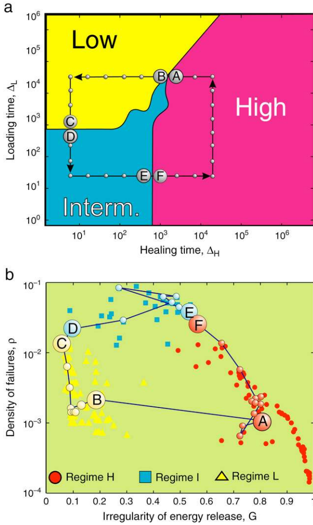
Fig. 11. Bifurcation diagram for the BDE seismic model: (a) rectangular path in the delay plane (\Delta_L, \Delta_H) ; and (b) the measures \mathcal{G} and \rho , calculated along the rectangular path shown in panel (a). The transition between points (A) and (B), i.e. between regimes H and L , is very sharp with respect to the change in irregularity \mathcal{G} of energy release, while almost negligible with respect to the change in failure density \rho . The colored circles, triangles, and squares in panel (b) correspond to synthetic catalogs from regimes H , I , and L , respectively; these catalogs are produced for the points indicated along the rectangular path in panel (a), as well as for many scatter points that lie on a uniform grid covering the entire regime diagram, with the same resolution in \Delta_H and \Delta_L as those along the path.
