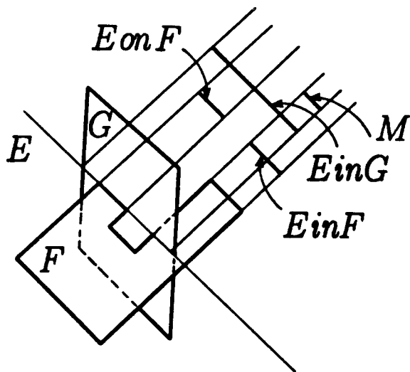
Figure 85 Edge/face operations.
