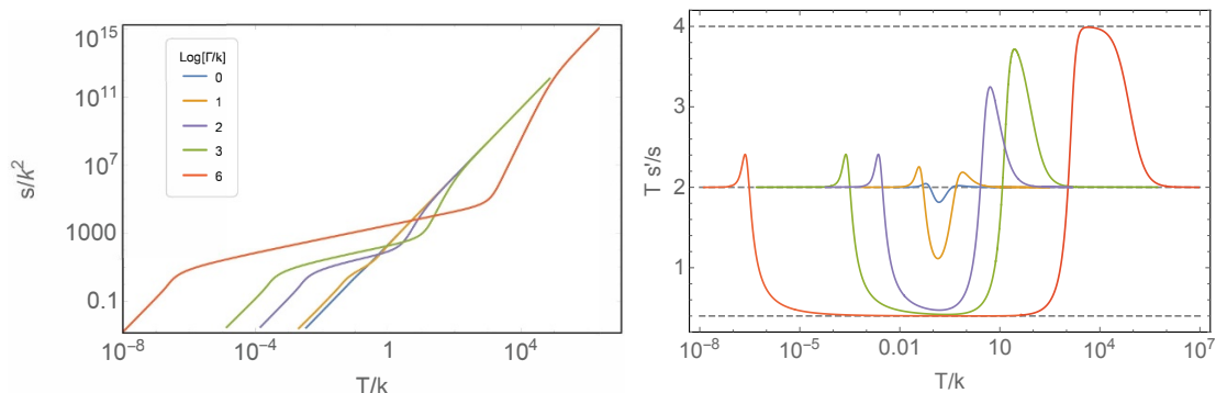
Figure 4. Behaviour of the entropy density, s , as a function of temperature, for various boomerang RG flows: blue ( \Gamma/k = 1 ), orange ( \Gamma/k = 10 ), purple ( \Gamma/k = 10^2 ), green ( \Gamma/k = 10^3 ) and red ( \Gamma/k = 10^6 ). In the UV and in the IR we have Ts'/s \rightarrow 2 , associated with AdS_4 . We also see, for large enough values of \Gamma/k , the appearance of two intermediate scaling regimes that are governed by the hyperscaling violation solutions which have Ts'/s = 4 and Ts'/s = 2/5 .
