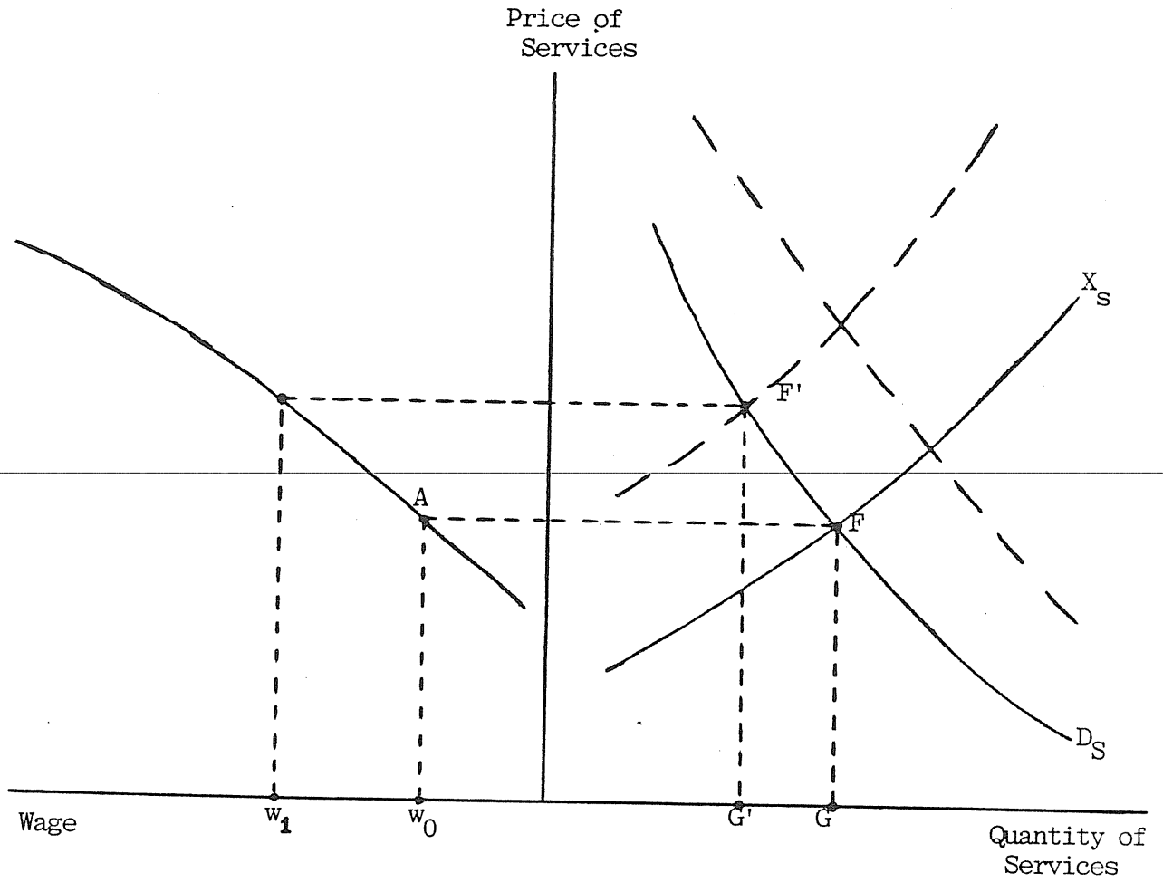
Figure 3: Effect of the Boom when Capital is Mobile between Two Sectors
