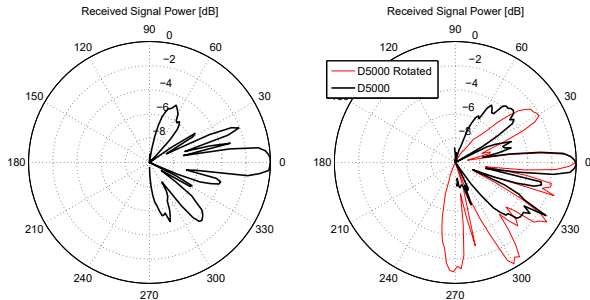
Figure 17: Laptop (left) and D5000 (right) beam patterns. Main lobe points always to 0 degrees.
