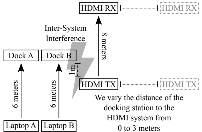
Figure 6: Interference analysis setup.
