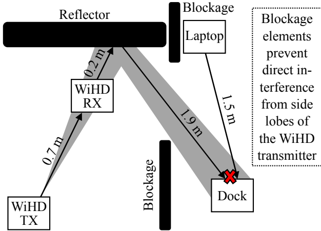
Figure 7: Reflection interference setup.
