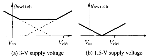
Figure 2: On-state conductance of the transmission-gate switch.
