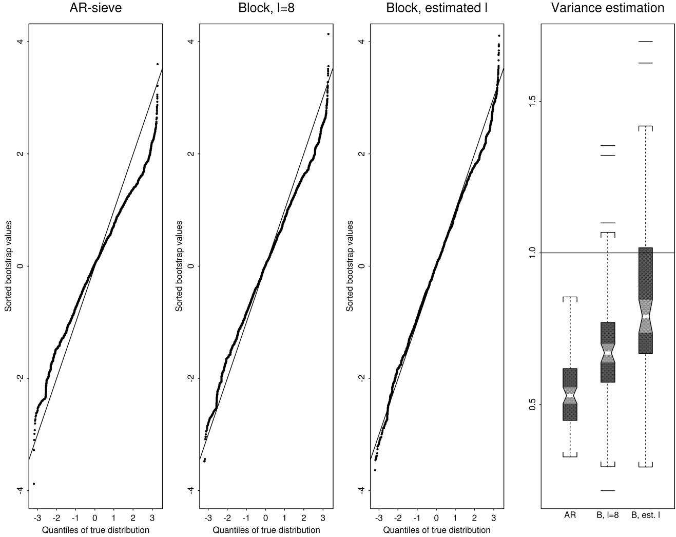
FIG. 6. Nonlinear model (4.4), n = 512 ; bootstrap distribution and variance estimation of (\hat{\theta} - \mathbb{E}[\hat{\theta}])/\sigma_n by (\hat{\theta}^* - \mathbb{E}[\hat{\theta}^*])/\sigma_n for \hat{\theta} = \text{med}(X_1, \dots, X_n) [ \sigma_n = (\text{Var}(\hat{\theta}))^{1/2} ]: (three left panels) QQ-plots with target indicated by the line; (right panel) boxplots with target indicated by the horizontal line. 100 simulation runs, 500 bootstrap replicates per simulation run.
