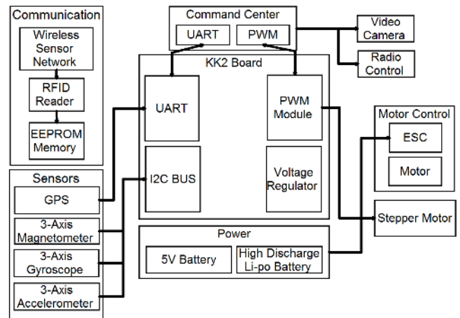
Figure 7: Electrical architecture
