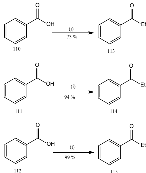
Scheme 20 Alkylation reaction
