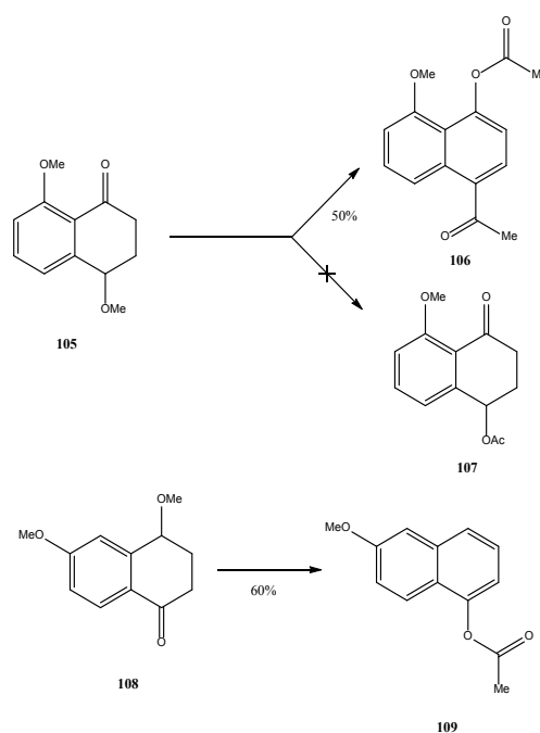
Scheme 19 Aromatization of tetralones
