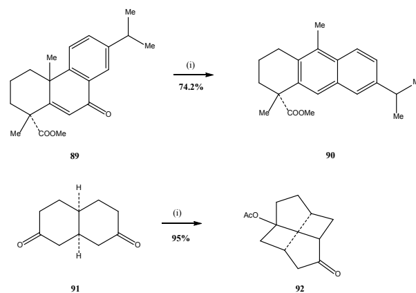
Scheme 17 Rearrangement of diketones
