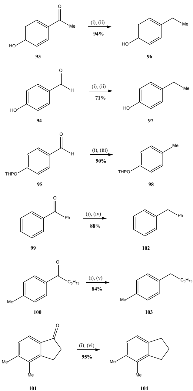
Scheme 18 Conversion of the aryl ketones into the corresponding hydrocarbons
