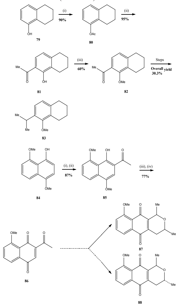
Scheme 16 Synthesis of quinones from Naphthol
