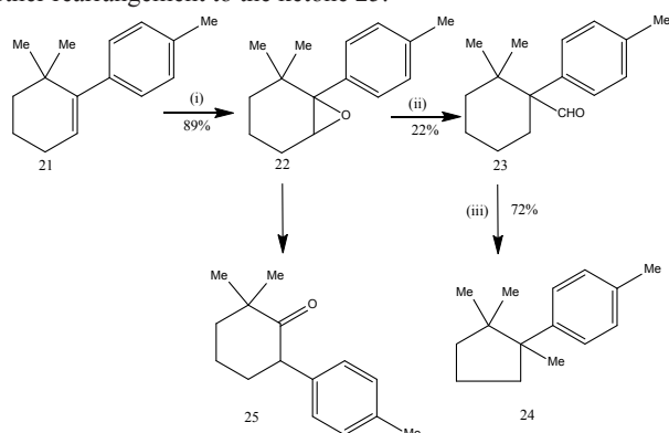
Scheme 6 Synthesis of cuprane
