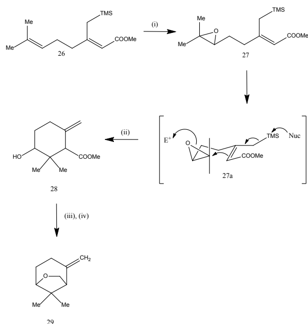
Scheme 7 Synthesis of ( \pm ) Karahana ether
