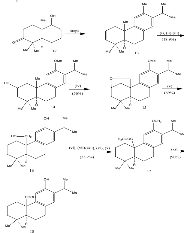
Scheme 4 Synthesis of pisiferic acid 18
