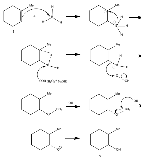
Scheme 2 Reaction mechanism for the formation of trans -2-methylcyclohexanol 2
