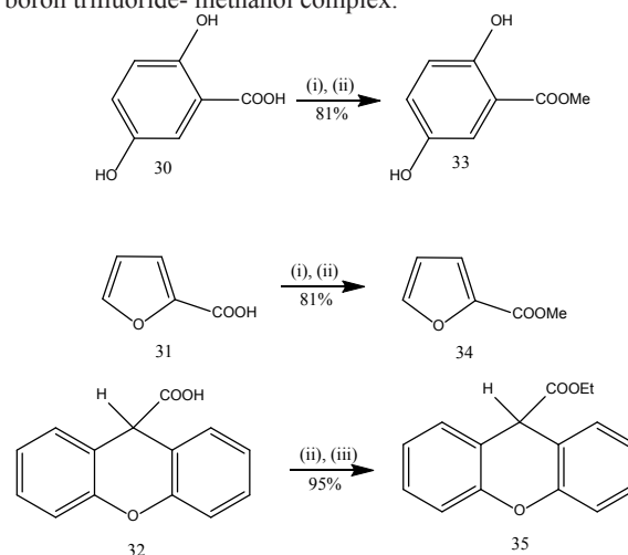
Scheme 8 Esterification of acids 32-35
