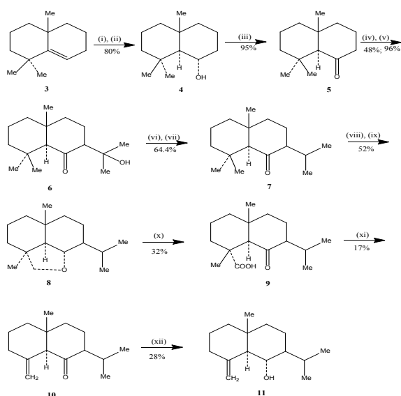
Scheme 3 Synthesis of eudesmone sesquiterpenes (±) junenol and (±)-acalomone
