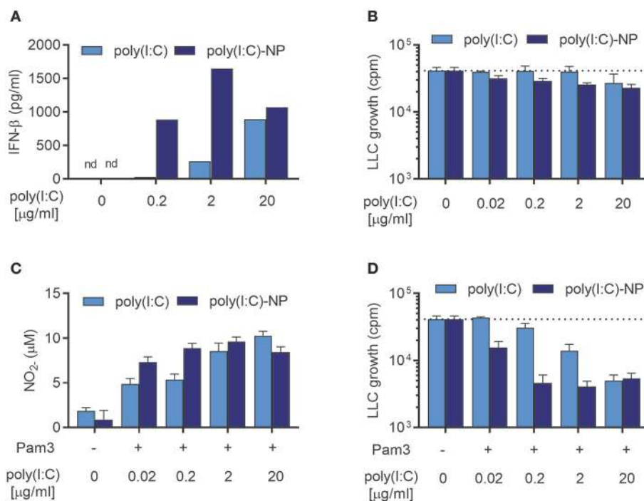
FIGURE 8 | Encapsulation of poly(I:C) into nanoparticles (poly(I:C)-NPs) potentiates the synergy of combined stimulation with Pam3CSK4 and poly(I:C) in the induction of antitumor BMDMs. (A) Production of IFN- \beta by BMDMs ( 6 \times 10^4 in 200 \mu L) stimulated with the indicated concentrations of poly(I:C) either in soluble form or encapsulated in nanoparticles (poly(I:C)-NPs) for 24 h. (B) Growth inhibition of LLC-cells ( 3 \times 10^3 ) in co-culture with BMDMs ( 6 \times 10^4 ), stimulated for 24 h with the indicated concentrations of either soluble poly(I:C) or poly(I:C)-NPs. (C) Production of NO by BMDMs ( 6 \times 10^4 ) treated for 24 h with the indicated concentrations of either soluble poly(I:C) or poly(I:C)-NPs alone or in combination with 100 ng/mL Pam3CSK4. (D) Growth inhibition of LLC cells in co-culture with BMDMs, stimulated as described in (C) . Data represent the means \pm SD of triplicate wells of one representative experiment out of two. nd, not detectable; Pam3, Pam3CSK4.
