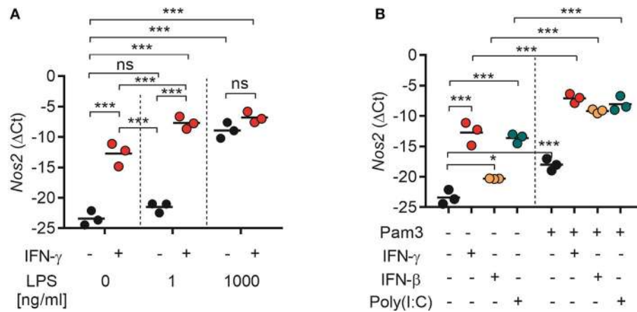
FIGURE 7 | Both type I and II IFNs synergize with TLR agonists for induction of Nos2 gene expression. BMDMs ( 4.5 \times 10^5 ) were stimulated for 24 h. Total RNA was reverse transcribed into cDNA and analyzed by RT-qPCR using primers specific for mouse Nos2 mRNA. (A) Nos2 expression in BMDMs treated with IFN- \gamma (40 ng/mL), or LPS at the indicated concentrations, or a combination of both. (B) Nos2 expression in BMDMs treated with IFN- \gamma (40 ng/mL), IFN- \beta (40 ng/mL), poly(I:C) (100 \mu g/mL), Pam3CSK4 (100 ng/mL), or the indicated combinations. Data are presented as means ( \Delta Ct) of duplicates for each of the three independent experiments. Each circle in the graphs represents the mean value from one experiment. P -values from a two-way ANOVA multiple comparison test is displayed as follows: * p < 0.05, *** p < 0.001; ns, not significant; Pam3, Pam3CSK4.
