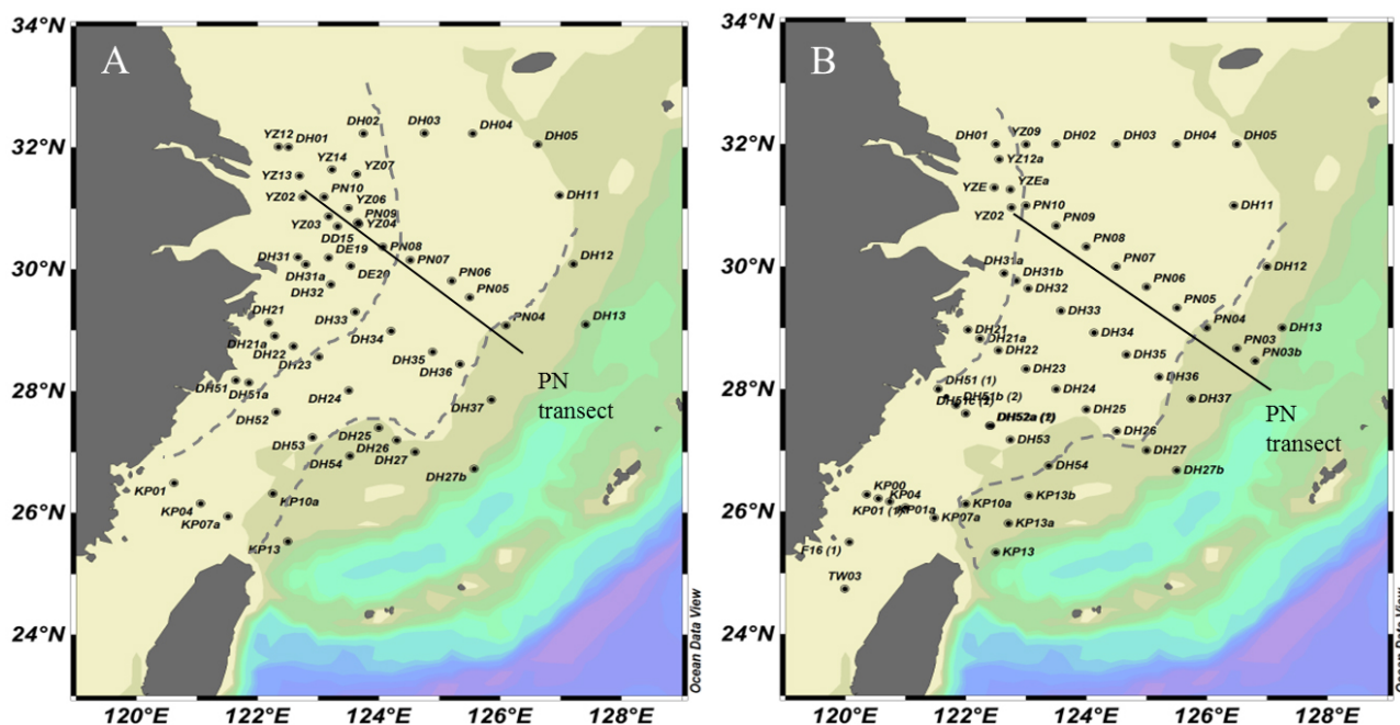
Fig. 1. Location of investigated stations in (A) summer and (B) winter. Plume, transitional, and Kuroshio regions were divided by the grey dotted lines. The PN transect is labeled as a black line.
