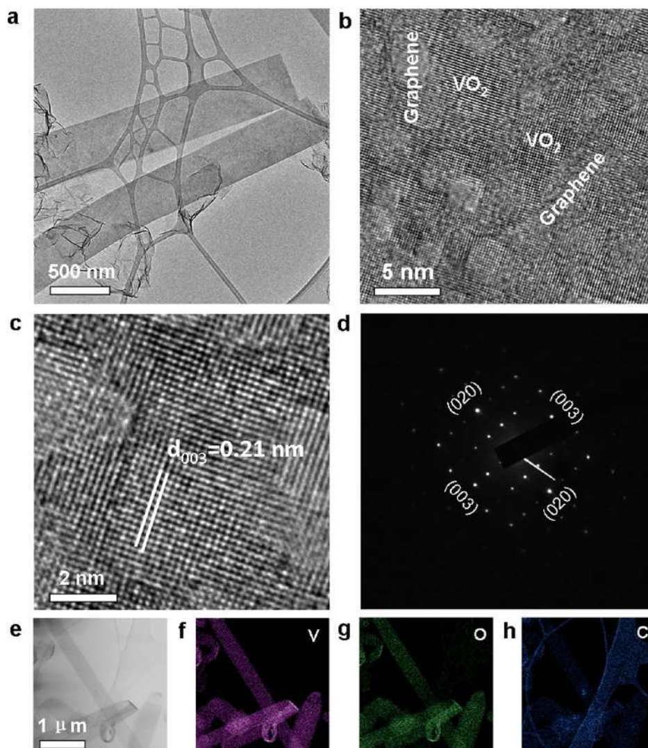
Figure 2. VO 2 -graphene ribbons. (a) Typical TEM image and (b,c) HRTEM images of VO 2 ribbons show the incontinuous graphene layers on the surface of well-crystalline ribbons. The exposed lattice fringes shown in part c has a spacing of 0.21 nm, corresponding to the (003) plane of VO 2 (B). (d) The representative diffraction patterns show well-defined arrays of dots, demonstrating the single crystalline feature of VO 2 (B) ribbons. (e) Scanning transmission electron microscopy (STEM) image and corresponding elemental mapping of (f) vanadium, (g) oxygen, and (h) carbon, indicating the homogeneous dispersion of V, O, and C in all of the ribbons.
