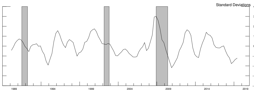
Figure 4: Dispersion index, NFCH^s , derived from predicted corporate default probability distribution
