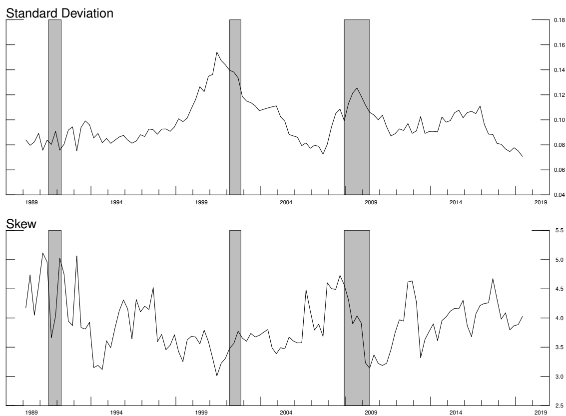
Figure 9: Unweighted Moments of the Corporate Default Probability Distribution
