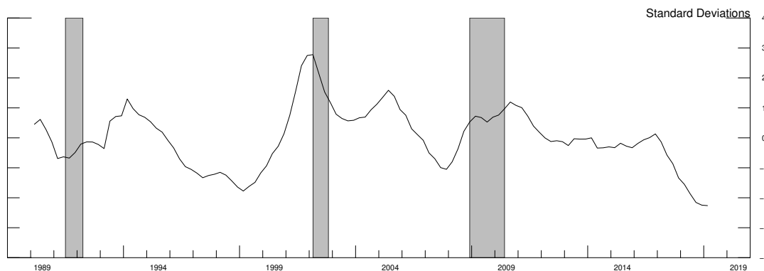
Figure 3: Level index, NFCH^m , derived from predicted corporate default probability distribution
