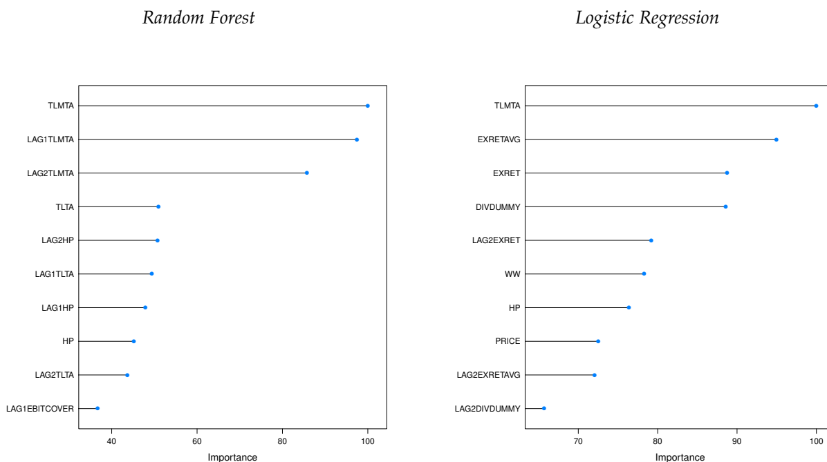
Figure 8: Variable Importance by Machine Learning Algorithm
