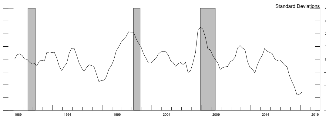
Figure 5: Ensemble index, NFCH , constructed as the average of NFCH^m and NFCH^s
