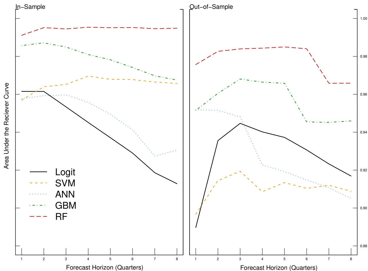
Figure 2: AUC by Machine Learning and Logistic Algorithms
