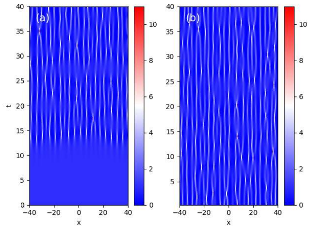
Figure 2. Numerical simulations of 1D-NLSE : Space-Time diagrams of |\psi(x, t)|^2 . (a) Noise-induced Modulational Instability of a plane wave. (b) Dynamics of the random phase bound N -SS (the initial condition |\psi(x, 0)|^2 is shown in the Fig. 1.a)
