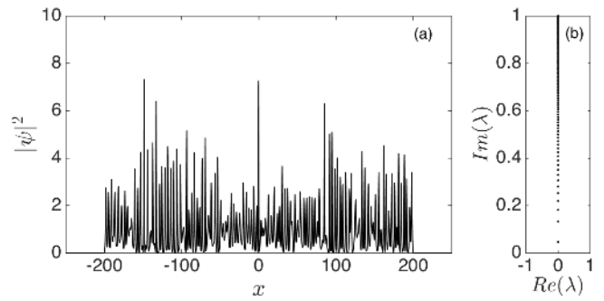
Figure 1. Example of one realization of 128-SS with random norming constant phases. (a) Intensity profile |\psi(x, t = 0)|^2 . (b) Soliton eigenvalues computed from Eq. (5).
