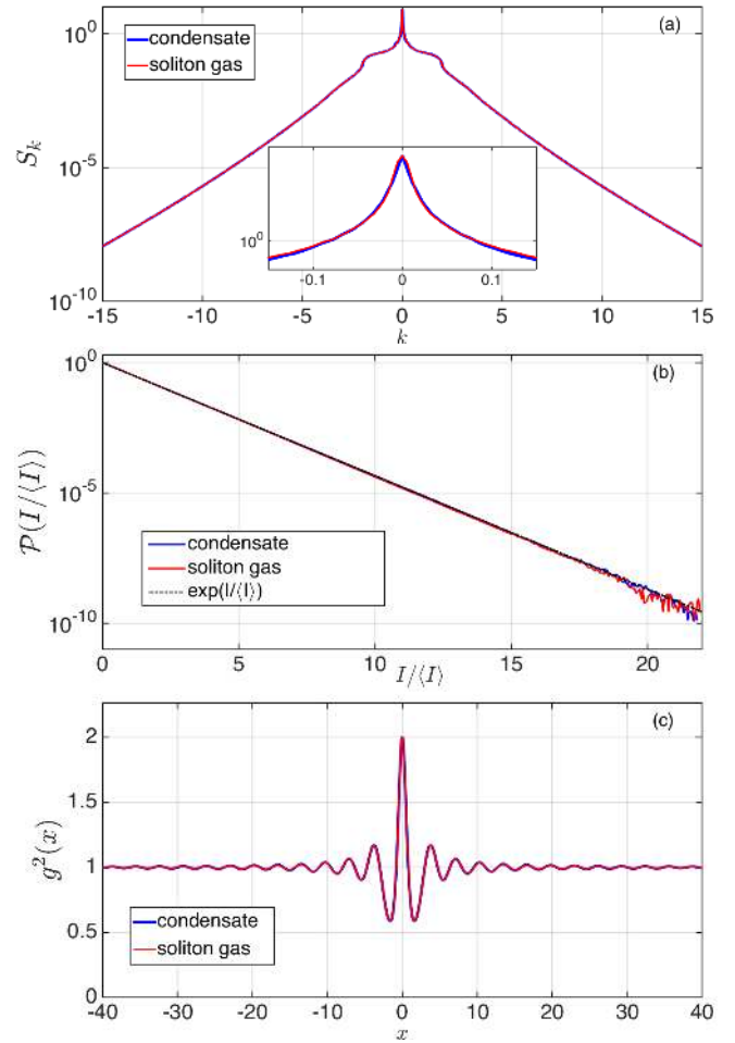
Figure 4. Comparison of ensemble averaged statistical characteristics of the asymptotic state of the MI development and of random phase 128-SSs. (a) Wave action spectrum S_k . (b) The PDF \mathcal{P}(I) . (c) Autocorrelation function of intensity (second order degree of coherence) g^{(2)}(x)
