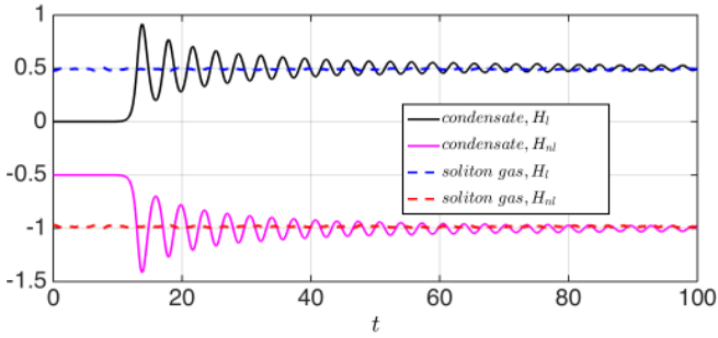
Figure 3. Time evolution of the ensemble-averaged kinetic \langle H_I(t) \rangle and potential \langle H_{nl}(t) \rangle energies for the noise-induced MI (black and magenta solid lines) and random phase SG (blue and red dashed lines).
