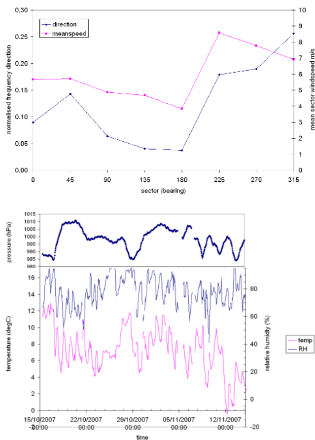
Fig. 2. Meteorological data measured using Vaisala WXT510 weather station at BT Tower during REPARTEE II. (a) Mean wind-speed and direction frequency data per 45^\circ sector. (b) Time series of temperature, relative humidity and pressure data for BT Tower.
