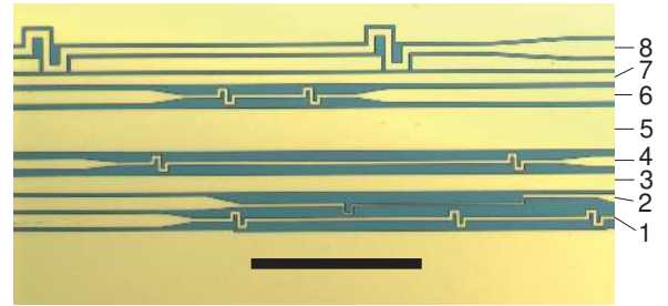
FIG. 1: (Color online) Optical microscope image of the central section of an atom chip. The chip hosts a series of micro-wires of various geometries for creating one-dimensional traps and box-shaped potentials. The length of the scale bar is 500 \mu\text{m} . The numbers at the right identify the atom chip wires and correspond to the numbers in Table I.
