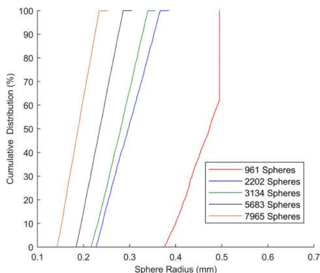
Fig. 5 Cumulative mass-based distribution of the spheres used in different pellet packing
