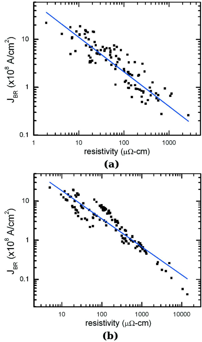
FIG. 3. (Color online) Breakdown current density vs resistivity; (a) shows a scatter plot with low-bias resistivity plotted on the x -axis—the R^2 for this fit is 74%; (b) shows a scatter plot for breakdown current density vs high-bias resistivity; the R^2 for this fit is 86%. The fit for both the plots is of the form J_{BR}=A\rho^{-B} where B=0.71 . If the breakdown mechanism was Joule heating, theory predicts that the exponent in the fit (b) should be 0.5; a steeper exponent in the fit indicates that the breakdown occurs faster for higher-resistivity GNRs, and might be indicative of higher defect densities contributing to faster electrical breakdown.
