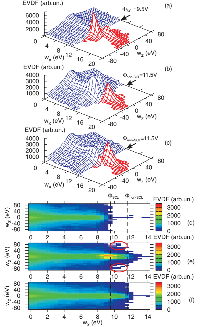
FIG. 4 (color online). EVDFs over v_x and v_z in the middle of the plasma 10 \text{ mm} < x < 15 \text{ mm} obtained (a), (d) in the SCL stage at t_1 = 9057 ns, (b), (e) in the beginning of the non-SCL stage at t_2 = 9095 ns, and (c), (f) in the end of the non-SCL stage at t_3 = 9269 ns (times t_{1,2,3} are marked by arrows in Fig. 2). Surfaces depicted by thin (blue) and bold (red) lines in (a), (b), (c) correspond to the electrons of the plasma bulk and the secondary electron beam, respectively. Panels (d), (e), (f) are the color maps of the plasma bulk EVDFs corresponding to the thin-line (blue) surfaces in (a,b,c), respectively. White areas in (d), (e), (f) contain no particles. Ovals in (e) mark areas which are replenished during the non-SCL stage. Graphs are plotted in energy coordinates, negative energy values correspond to propagation in the negative direction. Only parts of EVDFs moving in the positive x direction are shown.
