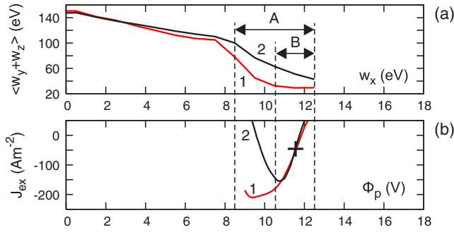
FIG. 5 (color online). (a) Average energy of motion of plasma bulk electrons in the direction parallel to the walls versus the energy of motion normal to the walls. The dependencies are obtained by averaging over particles in the middle of the plasma 10 \text{ mm} < x < 15 \text{ mm} . Region A corresponds to electrons escaping to walls during the SCL stage (the weakly confined electrons). Region B corresponds to the range of perturbations of the plasma potential in the system. (b) Total electron current at the wall x = H versus the plasma potential relative to the wall. The cross marks the actual average values of current J_e \approx -33.3 \text{ A/m}^2 and potential \Phi_p \approx 11.5 \text{ V} between times t_2 and t_3 . Curves 1 (red) are at t_2 = 9095 \text{ ns} , curves 2 (black) are at t_3 = 9269 \text{ ns} (same as t_{2,3} in Figs. 2 and 4).
