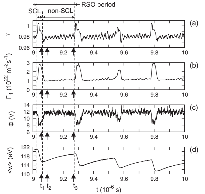
FIG. 2. Relaxation sheath oscillations. Temporal evolution of emission coefficient at x = H (a), primary electron flux at x = H (b), plasma potential at x = H/2 (c), and energy of an electron averaged over all particles (d). Dashed vertical lines mark the beginning and the end of the RSO period and the transition from SCL to non-SCL state. Arrows mark times t_1 = 9057 ns, t_2 = 9095 ns, and t_3 = 9269 ns when the EVDFs shown in Fig. 4 are taken. Dashed horizontal line in (a) marks a theoretical value of the critical emission coefficient \gamma_{cr} = 0.983 for a xenon plasma with a Maxwellian EVDF [2].
