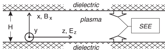
FIG. 1. Schematic diagram of the simulation model. Positions of the walls are x = 0 and x = H .
