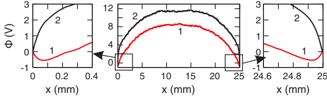
FIG. 3 (color online). Typical profiles of plasma potential during the SCL (curve 1, red) and the non-SCL (curve 2, black) regimes. The left and right panels show details of the middle panel in the near-wall regions. The walls are at x = 0 and x = 25 mm. Curve 1 (red) is at t = 9038 ns; curve 2 (black) is at t = 9076 ns.
