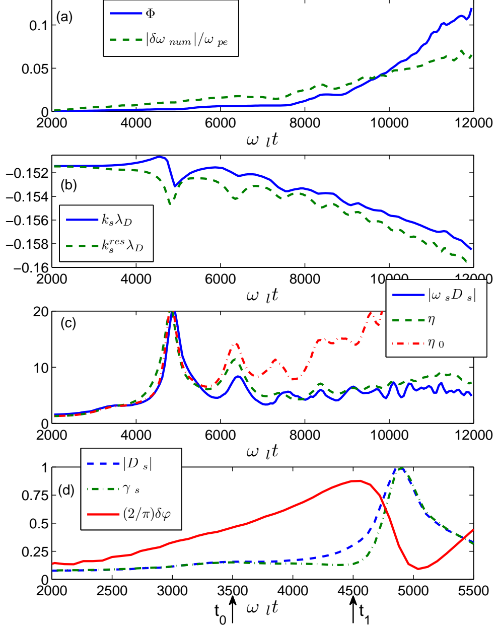
FIG. 3: (Color online) Numerical values for T_e=5 keV, k\lambda_D \approx 0.448 , and I_l=4 PW/cm 2 , measured at x = 173.5\lambda_l of, panel (a): \Phi (blue solid line) and |\delta\omega_{\text{num}}|/\omega_{pe} (green dashed line); panel (b): k_s (blue solid line) and k_s^{\text{res}} (dashed green line); panel (c): |\omega_s D_s| (blue solid line), \eta \equiv E_p/E_d (green dashed line) and \eta_0 \equiv \eta[k_s = k_s^{\text{lin}}] , normalized to their linear values; panel (d): |D_s| (blue dashed line) and \gamma_s (green dashed-dotted line) normalized to their maximum values, and (2/\pi)\delta\varphi (red solid line) vs. \omega_l t .
