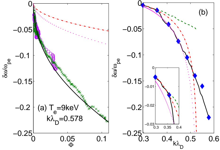
FIG. 2: (Color online) (a): \delta\omega_{\text{srs}} (black solid line), \delta\omega_{\text{D}} (red dash-dotted line), \delta\omega_{\text{MO}} (pink dots) and \delta\omega_{\text{num}} at x = 77\lambda_l (purple circles) and at x = 232\lambda_l (green crosses) for T_e=9 keV and I_l=8 PW/cm 2 . (b): \delta\omega_{\text{num}} (diamonds), \delta\omega_{\text{srs}} (black solid line), \delta\omega_{\text{free}} (green dashed line), \delta\omega_{\text{D}} (red dash-dotted line), and \delta\omega_{\text{MO}} (pink dotted line) vs. k\lambda_D when \Phi = 0.1 . Each numerical result is for a distinct run with a different T_e , and I_l=2 PW/cm 2 for T_e < 6 keV ( k\lambda_D < 0.485 ), I_l=4 PW/cm 2 for T_e=6 keV, I_l=6 PW/cm 2 for T_e=7 keV ( k\lambda_D \approx 0.519 ) and I_l=8 PW/cm 2 for T_e > 7 keV.
