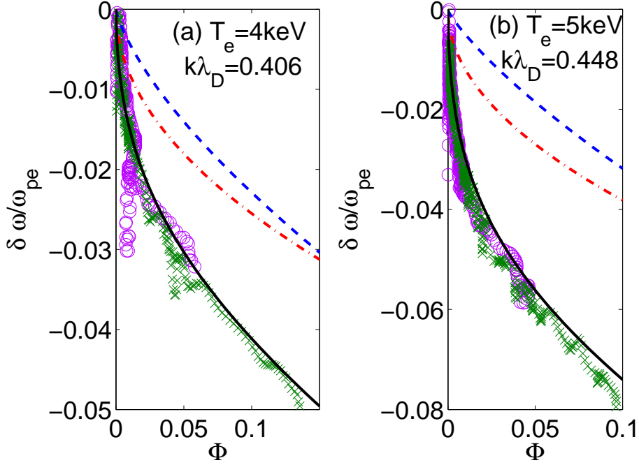
FIG. 1: (Color online) \delta\omega_{\text{srs}} (black solid line), \delta\omega_{\text{free}} (blue dashed line), \delta\omega_D (red dash-dotted line), \delta\omega_{\text{num}} at x = 77\lambda_l (purple circles) and at x = 193\lambda_l (green crosses) for I_l = 2 \text{ PW/cm}^2 and (a) T_e = 4 \text{ keV} , and (b) T_e = 5 \text{ keV} .
