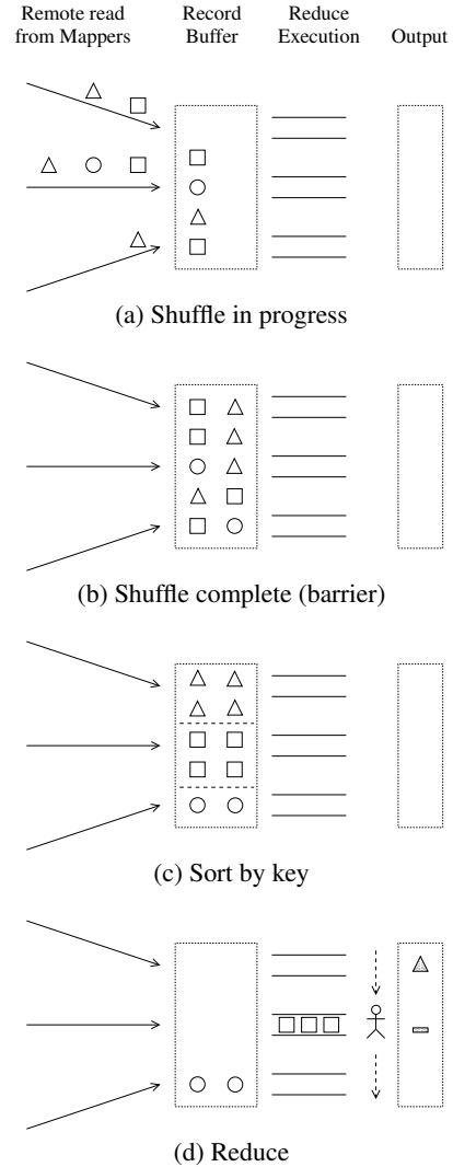
Figure 2: MapReduce Shuffle and Reduce stages as seen at a Reduce node. Each record is shown as a shape representing its key. This shape is also used to show the key for the Reduce output. Partial output is represented with a small portion of the shape.
