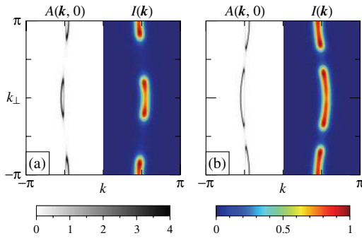
FIG. 4 (color online). Comparison of the zero-energy spectral function A(\mathbf{k}, 0) at T = 0 with the expected ARPES intensity I(\mathbf{k}) calculated assuming a k -space resolution of 0.04\pi , an energy resolution 0.004t , and an energy integration window \delta E = 0.01t . The self-energy parameters are taken from Fig. 3(b) for t_{\perp} = 0.42 (a) and t_{\perp} = 0.46 (b).
