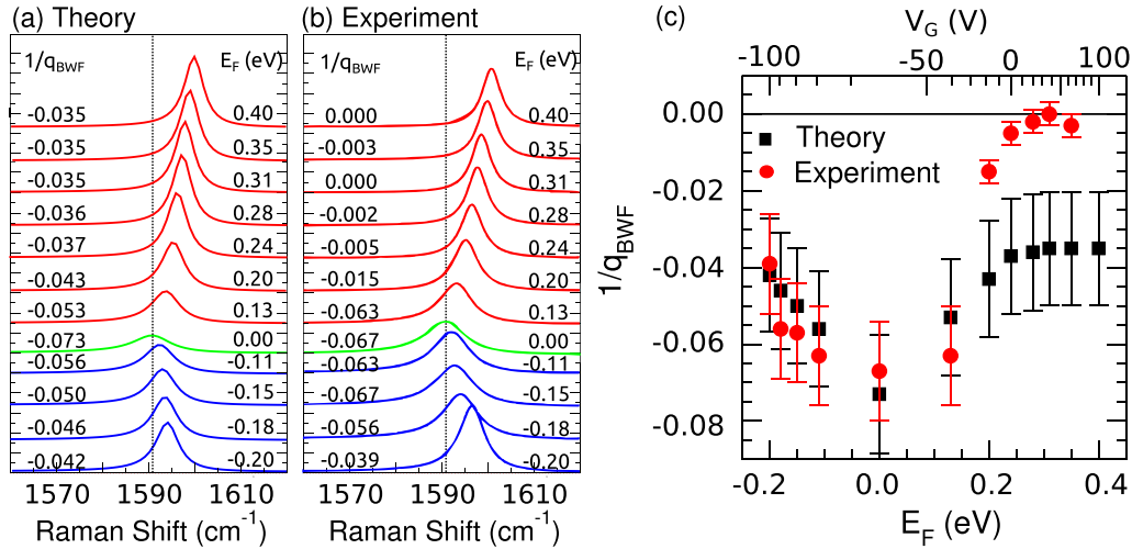
FIG. 4. (Color online) Comparison between (a) the calculated results (this work) and (b) the experimental results taken from Ref. [9] for the G -band Raman intensity as a function of the Raman shift, which is plotted for various values of E_F in the range -0.20 \leq E_F \leq 0.40 eV. The values of 1/q_{\text{BWF}} obtained from the calculation and the experiment are also given on each plot. (c) Comparison of the BWF asymmetric factor 1/q_{\text{BWF}} as a function of E_F and gate voltage V_G between theory (squares) and experiment (circles). Both the linewidth and the phonon peak frequency shift due to the Kohn anomaly effect are fitted from the experimental results in Ref. [9].
