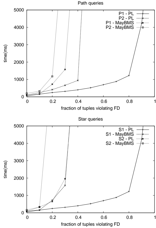
Figure 6: Varying the number of offending tuples.
