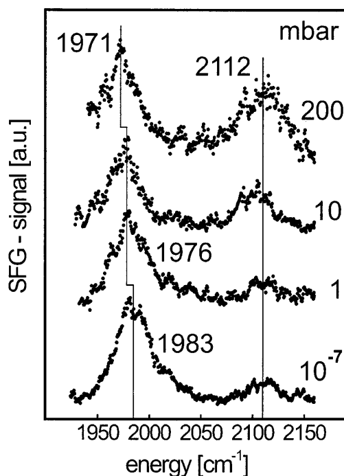
FIG. 3. SFG spectra of CO adsorption on a Pd/Al 2 O 3 model catalyst at 190\text{ K} ( 6\text{ nm} Pd particles grown at 300\text{ K} ). Because of the more ordered structure of the 6\text{ nm} Pd particles, at low pressure the fraction of on-top CO is smaller than on the 3\text{ nm} Pd particles.
