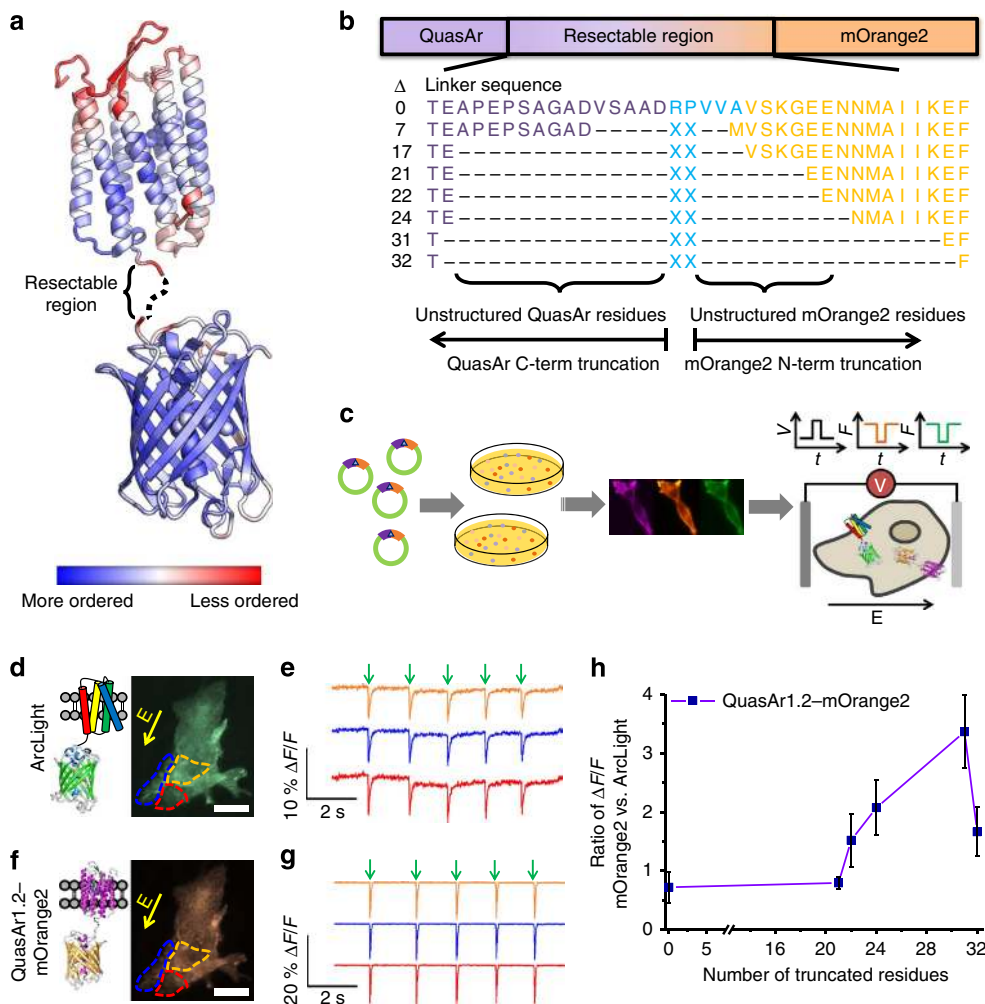
Figure 2 | Directed evolution of an eFRET GEVI. (a) A model of QuasAr-mOrange2 constructs, represented by the crystal structures of Arch-2 (PDB ID 2EI4) ref. 26 and mOrange (PDB ID 2H5O) 27 . The color scale represents the degree of order in the crystal structure, as reported by the B-factor. Less-ordered regions are presumed more dispensable. (b) Design of linker truncation libraries. QuasAr1.2, the best available variant at the time of the screen, was used as the electrochromic quencher. (c) Hierarchical screen of truncated linker libraries for eFRET GEVIs. Constructs were first screened in E. coli for mOrange2 brightness and then screened for membrane trafficking in HEK cells. Voltage sensitivity was then tested via field stimulation in HeLa cells co-expressing the eFRET GEVI, ArcLight (as an internal control), and Kir2.1 (to lower the resting voltage to -60\text{ mV}^{42} ). (d) ArcLight fluorescence of three HeLa cells. Yellow arrow indicates direction of the applied electric field. Scale bar, 25\ \mu\text{m} . (e) Fluorescence intensity traces of the three regions shown in d. (f) mOrange2 fluorescence from the same cells shown in d. (g) Response of mOrange2 fluorescence during stimulation as in e. Fluorescence traces show single-trial measurement of cells imaged at 100 frames per second. (h) Effect of linker length on voltage sensitivity in QuasAr1.2-mOrange2. For each linker length the most sensitive eFRET GEVI construct was compared with ArcLight measured in the same cells. Error bars represent s.d. over n = 15\text{--}20 cells in the ratio \Delta F/F .
