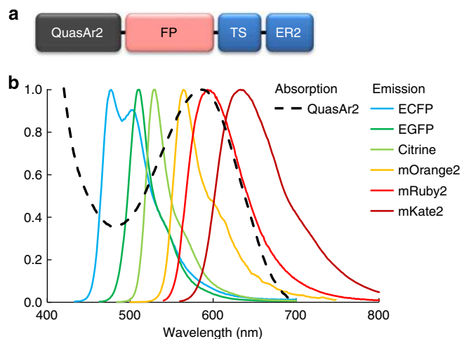
Figure 3 | Spectral overlap of fluorescent proteins with QuasAr2 absorption. (a) eFRET GEVI domain structure. (b) Overlay of the emission spectra of the fluorescent protein donors with the absorption spectrum of the QuasAr2 electrochromic quencher.
