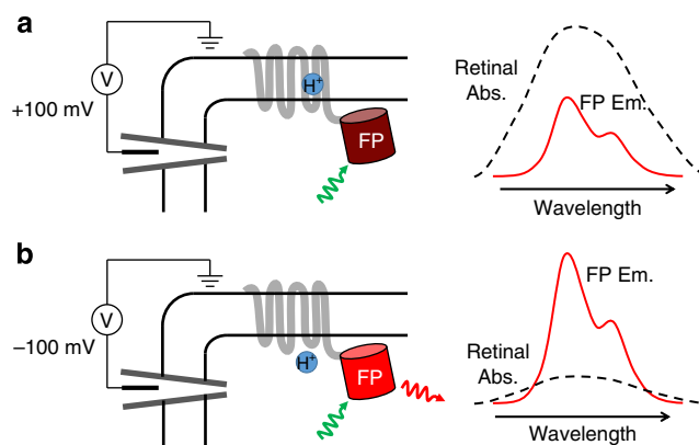
Figure 1 | Proposed mechanism of voltage-dependent fluorescence in eFRET GEVIs. Voltage controls the protonation, and thereby the absorption spectrum, of the Schiff base joining the retinal to the protein scaffold. (a) At a depolarizing (positive) voltage, the microbial rhodopsin has a protonated retinal Schiff base, which absorbs strongly with a peak near 600 nm. The retinal absorption quenches the fluorescence of the appended fluorescent protein (FP). (b) At hyperpolarizing (negative) voltages, the fluorescence is not quenched. Spectra shown are cartoons to illustrate mechanism.
