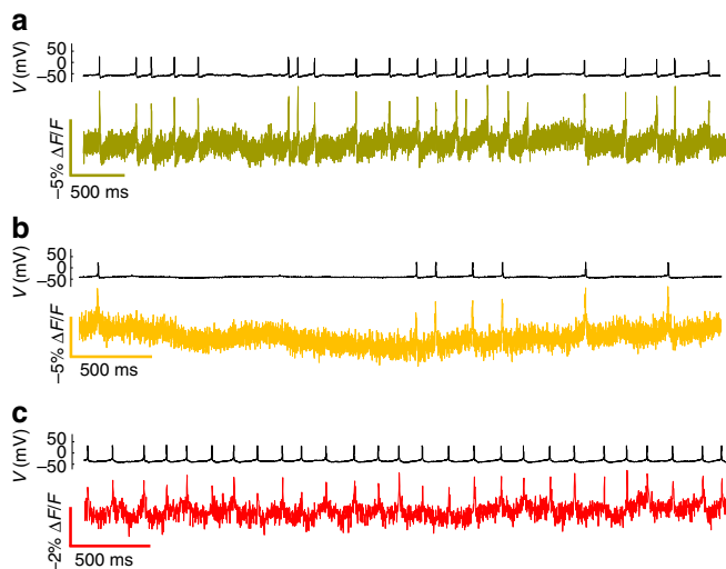
Figure 6 | Optical recording of spontaneous neuronal firing with eFRET GEVIs. In neurons synaptically coupled to a spontaneously active circuit, the (a) Citrine, (b) mOrange and (c) mRuby2 eFRET GEVIs clearly revealed single APs. Patch clamp voltage recordings are shown above optical recording traces. All recordings were acquired with laser illumination ( 3\text{ W cm}^{-2} ) at an exposure time of 2 ms. Fluorescence traces are presented without temporal filtering. The optical recordings have been corrected for photobleaching with a linear fit.
