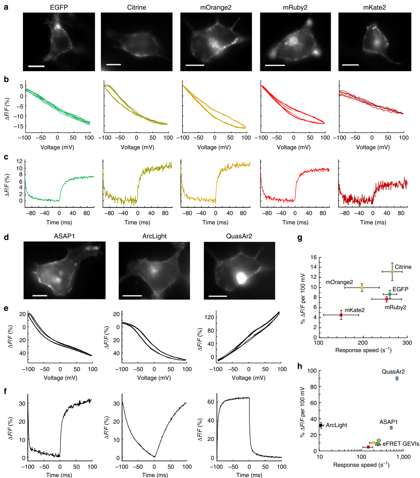
Figure 4 | Voltage sensing with GEVIs in HEK293 cells. Voltage response of eFRET GEVI reporters are shown in (a–c) and voltage responses of comparison GEVIs are shown in (d–f). (a,d) Fluorescence images of HEK cells expressing GEVI reporters. Scale bars, 10 \mu\text{m} . (b,e) Fluorescence as a function of membrane voltage, normalized to fluorescence at V = -70 mV. Many eFRET-based GEVIs showed a small amount of hysteresis. Each trace is a single trial with 100 ms exposures. (c,f) Fluorescence response to a step in membrane voltage from -70 mV to +30 mV. Each trace is averaged over 20–30 trials with 1 ms exposures. All data were acquired with laser illumination ( 3\text{ W cm}^{-2} for eFRET, ASAP1 and ArcLight GEVIs, 200\text{ W cm}^{-2} for QuasAr2). No temporal filtering was applied. Fluorescence traces were corrected for photobleaching. (g) Quantification of eFRET GEVI sensitivity and speed. Voltage sensitivity of eFRET GEVIs approximately corresponds to the degree of spectral overlap between the emission of the GEVI and the absorption of QuasAr2. (h) eFRET GEVI sensitivity and speed in the context of other GEVIs. Response speed was defined as the inverse of the time to reach 50% of steady-state response to a voltage step from -70 mV to +30 mV. Data in (g) and (h) represents an average of n = 6 –9 cells for each construct. Error bars represent s.e.m.
