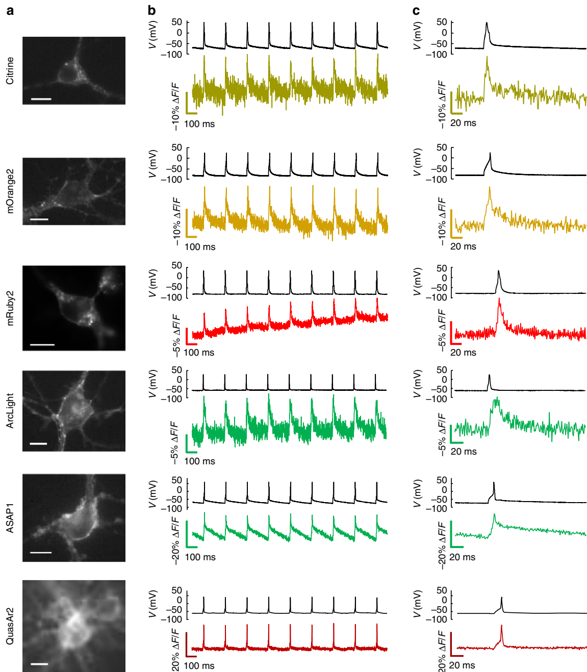
Figure 5 | Single-trial recording of neuronal APs with GEVIs. Each GEVI construct was expressed in primary rat hippocampal neurons under a CaMKII \alpha promoter. APs were induced by current injections through a patch pipette. (a) Images of neurons expressing the indicated GEVI. Scale bars, 10 \mu m. (b) Simultaneous patch clamp and fluorescence recordings of AP waveforms. All recordings were acquired with laser illumination ( 3 \text{ W cm}^{-2} for eFRET, ASAP1, and ArcLight GEVIs, 200 \text{ W cm}^{-2} for QuasAr2) at an exposure time of 1 ms. Fluorescence traces are presented without temporal filtering nor correction for photobleaching. All but the QuasAr2 recording have been inverted (hence photobleaching appears as an upward trend in the mRuby2 trace). Recordings are representative traces from 5–11 cells recorded for each construct. (c) Close-up showing single trial, unfiltered, electrically and optically recorded AP waveforms.
