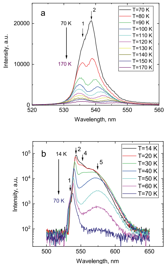
Figure 1. X-ray luminescence spectra of a CsPbBr 3 crystal measured at different temperatures. For better visualisation of changes the spectra are presented for two ranges of temperatures (a) 70–170 K (in linear scale) and (b) 14–70 K (in logarithmic scale).
