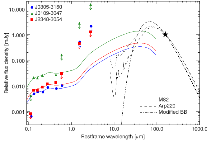
Figure 3. Spectral energy distributions (SEDs) of the three VIKING quasars, normalized to 1 mJy at 158 \mu\text{m} in the rest frame. The rest-frame UV to near-infrared data points are taken from Venemans et al. (2013) and from the Wide-field Infrared Survey Explorer (WISE, Wright et al. 2010). We fitted the quasar template of Richards et al. (2006) to the short-wavelength ( \lambda_{\text{obs}} < 30 \mu\text{m} ) data points of each quasar. The three models used in this paper to model the far-infrared emission are shown by the dotted line (M82 template), dashed line (Arp 220 template), and dotted–dashed line (modified blackbody).
