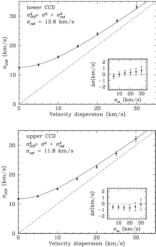
Fig. 1. The points with error bars are the average, raw velocity dispersion measurements ( \sigma_{\text{CCF}} ) obtained from 7 different template stars whose spectra were broadened to simulate the different input velocity dispersion ( \sigma_{\text{in}} values). The solid line is from Eq. (1) which is also displayed in each panel. The two diagrams are for the lower and upper CCDs of UVES, which have different \sigma_{\text{ref}} values. The inserts show the difference between the obtained and input true velocity dispersions as a function of input velocity dispersion.
