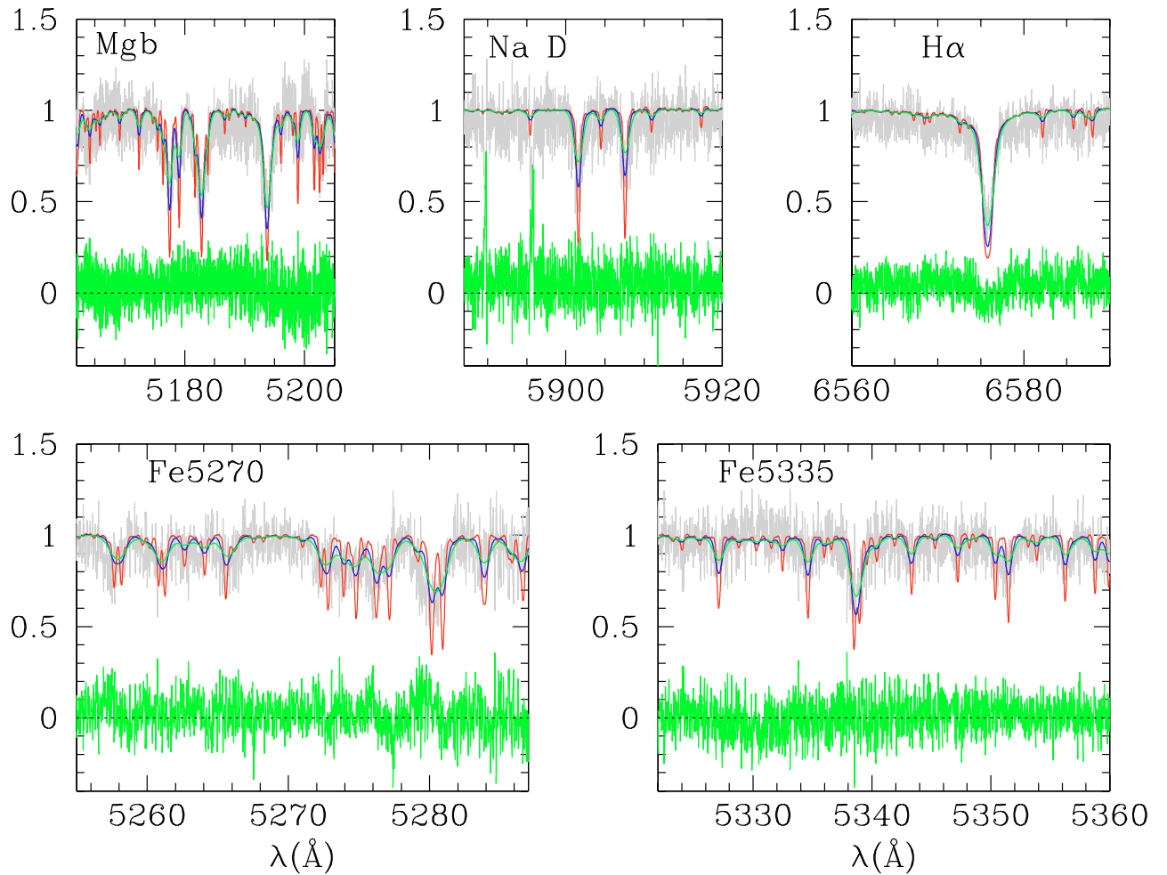
Fig. 4. The spectrum of HGHH92-C7 plotted in gray showing the spectral regions around some of the prominent absorption line features: Mgb, Na D, and H \alpha in the upper panel and Fe5270 and Fe5335 features in the lower panel . Overplotted are spectra of HD 103295 star broadened to simulate velocity dispersion of 5 (red line), 15 (blue), and 25 km s -1 (green). The best fitting template is the one widened by 25 km s -1 in agreement with 24.1 \pm 1.6 km s -1 obtained by cross-correlation (Table 4). The differences (template-GC) are shown at the bottom of each panel, demonstrating the goodness of the fit for the template broadened with \sigma = 25 km s -1 . (See the electronic edition of the journal for the colour version of this figure.)
