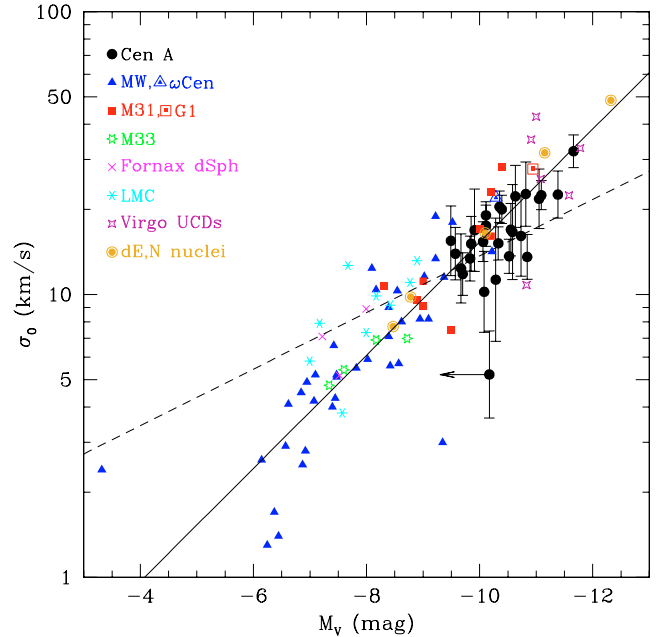
Fig. 7. Central velocity dispersion versus absolute V band magnitude relation for globular clusters in NGC 5128 (Cen A; black filled circles, this work). We compare it with old ( age > 10 Gyr) clusters in Local Group galaxies, as well as with transition objects between globular clusters and dwarf galaxies, UCDs/DGTOs from the work of Haşegan et al. (2005) and nuclei of dwarf ellipticals in Virgo (Geha et al. 2002). The sources of data for the Local Group clusters are as follows: the Milky Way, Fornax dSph and LMC clusters are from McLaughlin & van der Marel (2005), M 31 from Dubath & Grillmair (1997), M 33 from Larsen et al. (2002), G1 cluster data are from Meylan et al. (2001) and \omega Cen from Meylan et al. (1995). For clarity error-bars are omitted for all but our data. They include the uncertainties in the correction from observed to central \sigma . The outlying cluster from our sample, R01-122 has its luminosity overestimated due to probable blend with foreground stars, as indicated by the arrow. The dashed line is the Faber-Jackson relation (Faber & Jackson 1976) for bright ellipticals, while the solid line shows the best fit relation for Galactic globular clusters from McLaughlin & van der Marel (2005). (See the electronic edition of the journal for the colour version of this figure.)
