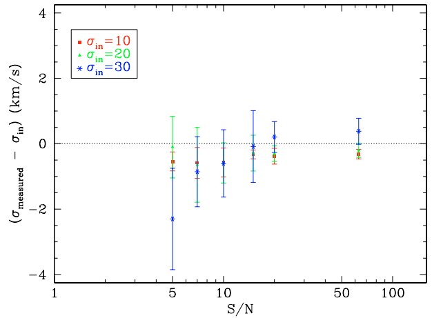
Fig. 3. Difference between the measured and simulated velocity dispersions as a function of S/N of the spectra. These simulations are based on 7 randomly selected template stars whose spectra were broadened by convolving them with Gaussians with widths of 10, 20, and 30 \text{ km s}^{-1} and had S/N degraded to simulate noisy spectra, closer to globular cluster targets. (See the electronic edition of the journal for the colour version of this figure.)
