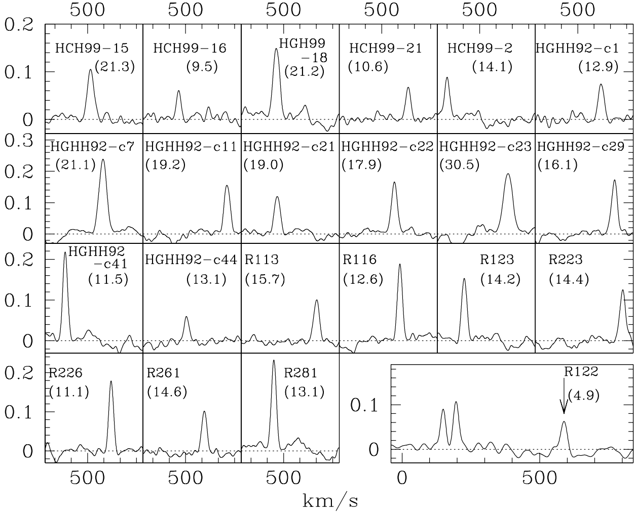
Fig. 5. The CCFs for all the clusters observed with UVES. The derived velocity dispersion is given in parenthesis next to the name of each cluster. The x -axis scale has been corrected for the relative velocity shift between the template star and the cluster so that the peak of the CCFs corresponds to the heliocentric velocity of the cluster. The x -axis displays one tick for every 100 km s -1 . All the CCFs show a single well-defined Gaussian peak, except for R122, which has additional peaks at velocities 59 and at 114 km s -1 due to contamination by Galactic foreground stars.
