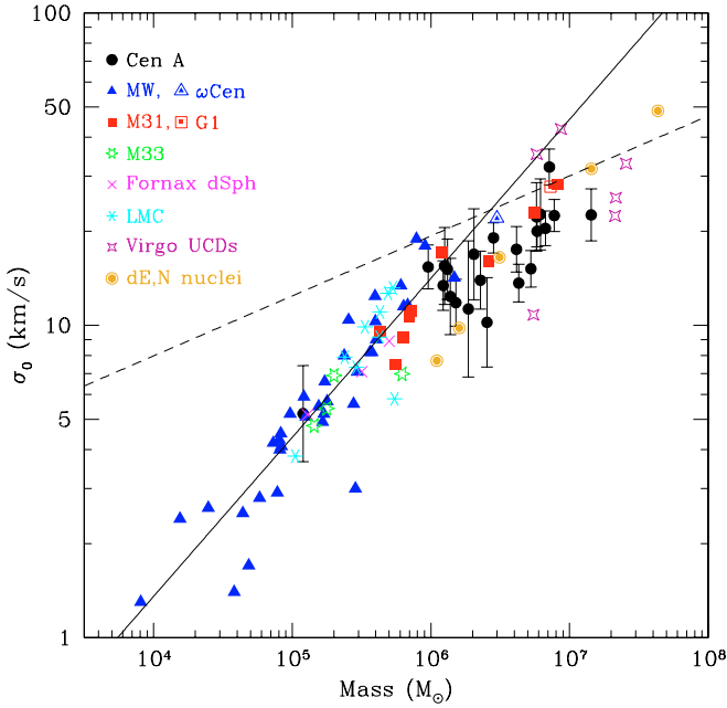
Fig. 8. Central velocity dispersion plotted as a function of mass. For the literature sources for the clusters from the Local Group galaxies and UCDs/DGTOs and dE,N nuclei from Virgo clusters see caption of Fig. 7. Solid line shows the virial theorem for globular clusters and the dashed line is a dependence between mass and \sigma for bright elliptical galaxies (Eqs. (12) and (13) from Håeghan et al. 2005). (See the electronic edition of the journal for the colour version of this figure.)
