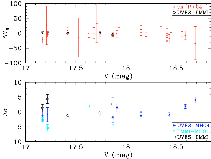
Fig. 6. Comparison of the measurements from the literature and our results, as well as a comparison between UVES and EMMI measurements for the clusters in common. In the upper panel we plot the difference between radial velocity and in the lower panel velocity dispersion differences as a function of magnitude. In both panels the open circles are used to compare UVES and EMMI measurements. The filled triangles compare radial velocities with those of Peng et al. (2004a, P+04). In the lower panel our velocity dispersions are compared with those of Martini & Ho (2004, MH04) for clusters observed with UVES (asterisks) and EMMI (open squares) separately. (See the electronic edition of the journal for the colour version of this figure.)
