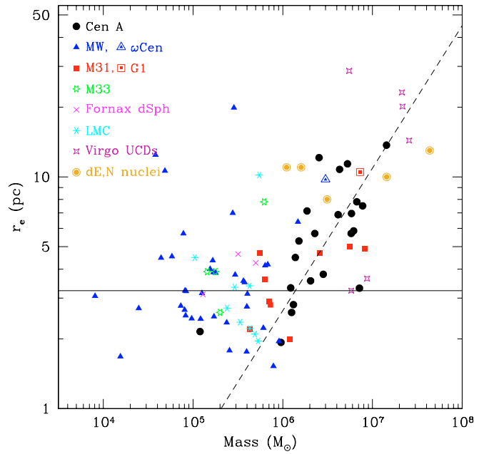
Fig. 10. Same as Fig. 8, but for effective (half-light) radius as a function of mass. The solid line shows the median r_e = 3.2 pc for Galactic globular clusters, while the dashed line shows the dependence between mass and effective (half-light) radius for bright elliptical galaxies (Eq. (12) from Håeghan et al. 2005). (See the electronic edition of the journal for the colour version of this figure.)
