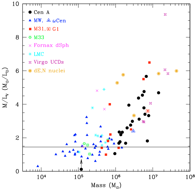
Fig. 9. Same as Fig. 8, but for mass-to-luminosity as a function of mass. The solid line shows the average dynamically determined M/L = 1.45 for a sample of Galactic globular clusters (McLaughlin 2000). (See the electronic edition of the journal for the colour version of this figure.)
