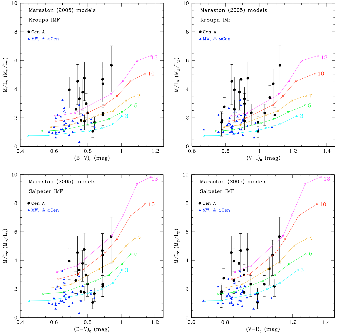
Fig. 11. The measured M/L ratios as a function of de-reddened (B - V) (left) and (V - I) (right) colours for our sample of clusters in Cen A. Together with the old globular clusters in the MW, they are compared to expected values from the SSP models of Maraston (2005) computed for two different IMFs, as shown in each panel. The ages of the theoretical predictions are shown on to the right of the curves. The model colours (open squares) from blue to red are for the following metallicities: [Z/H] = -2.25, -1.35, -0.33, 0.0, +0.35, and +0.67 dex. The colours of the MW clusters are taken from Harris (1996) web 2 catalogue. (See the electronic edition of the journal for the colour version of this figure.)
