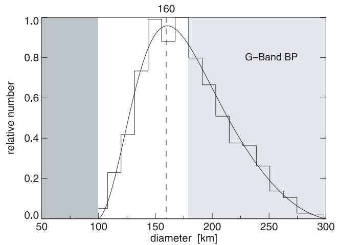
Fig. 6. Diameter histogram for 1528 inter-granular G -band bright points fitted by a polynomial; light grey indicates the resolution range of an ideal 45 cm telescope; dark grey visualizes sizes beyond the resolution limit achieved.
