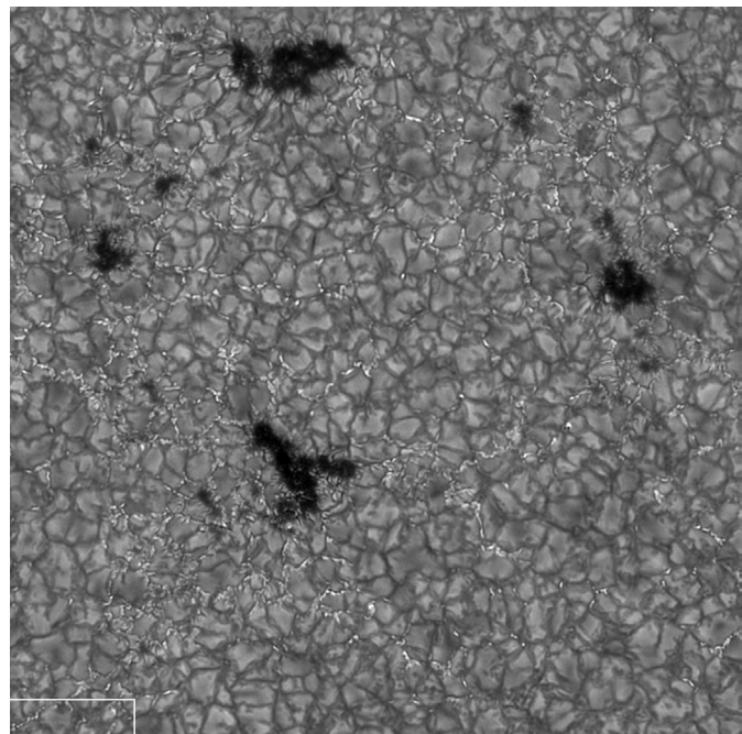
Fig. 1. Speckle reconstructed G -band image of an active region at 9°N, 8°W, taken with the 1 m SST on July 14, 2003; field of view: 57 arcsec × 57 arcsec; the lower left rectangle marks the sub-field in Fig. 2.
