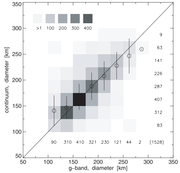
Fig. 5. Two dimensional diameter histogram of 1528 inter-granular bright points recognized in the G -band (abscissa) and in the continuum image (ordinate); the gray-scales give the lower boundary of the number density intervals; the total numbers of igBP for each sizebin is indicated; circles give the weighted means, vertical bars the \pm 1\sigma deviations.
