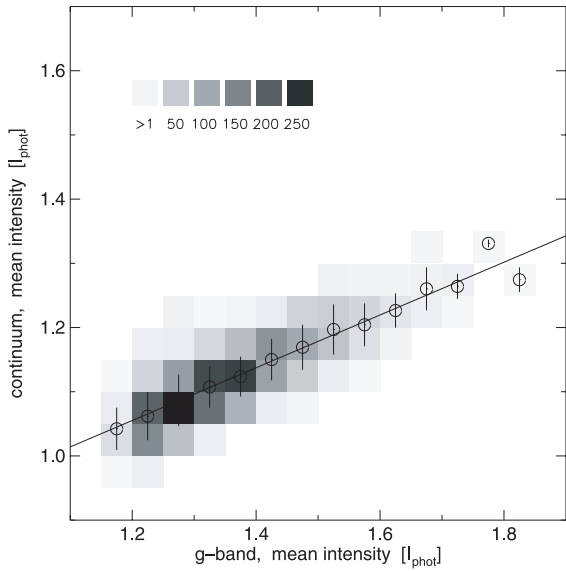
Fig. 3. Two dimensional histogram of the mean intensity of 1528 inter-granular bright points recognized in the G -band (abscissa) and in the continuum image (ordinate); the gray-scales give the number density of each data point; circles give the weighted means, vertical bars the \pm 1\sigma deviations.
