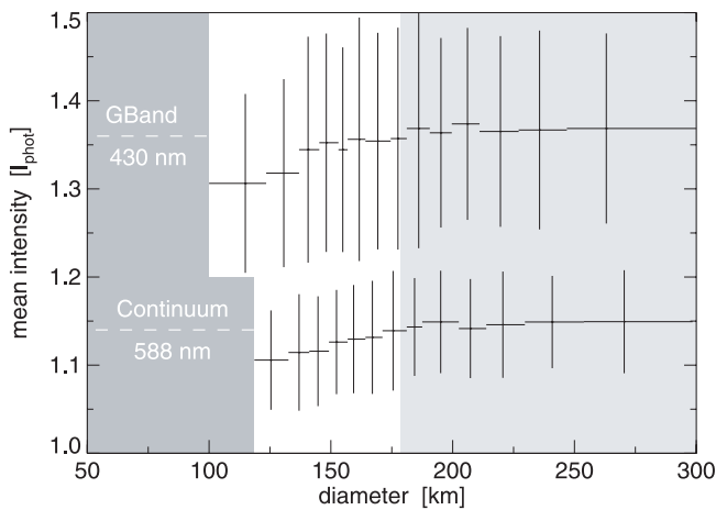
Fig. 4. Intensity-diameter relation of inter-granular features recognized in the G -band (upper) and in the continuum (lower part); x -bars mark samples of equal statistical weight; y -bars give standard deviations; light grey indicates the resolution range of an ideal 45 cm telescope; dark grey visualizes sizes below the SST's resolution; dotted lines give the total means.
