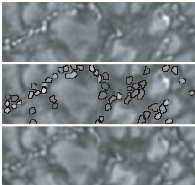
Fig. 2. Speckle reconstructed G-band ( upper ) and simultaneous 587 nm continuum ( lower ) images of a 9.6 \text{ arcsec} \times 3.0 \text{ arcsec} ( 7.1 \text{ Mm} \times 2.2 \text{ Mm} ) sub-field (rectangle at the lower left in Fig. 1); the middle panel shows the segmented intergranular features recognized in the G-band image (including even faintest ones for the tests explained in 4.2.b).
