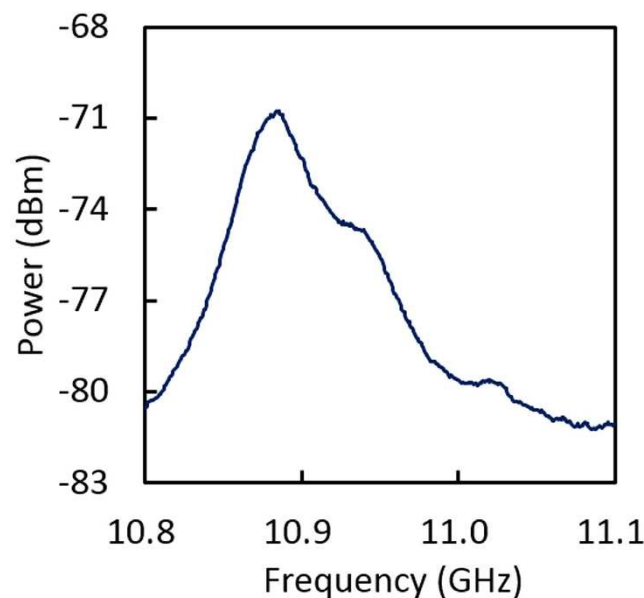
Figure 5. Measured BGS in the outer core of the MCF, overlapped with those in the SMF-1 and SMF-2.
