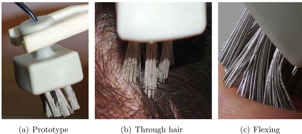
Figure 1. The silver-coated polymer bristles prototype
