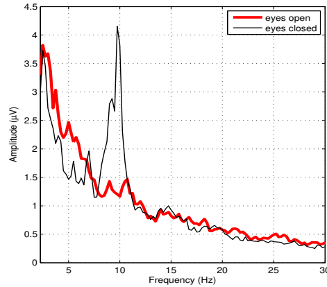
Figure 4. Spectra of the EEG signal recorded with the prototype for the eyes open/eyes closed conditions, averaged over all subjects with available data. It shows a peak at 10 Hz for the eyes closed condition.
