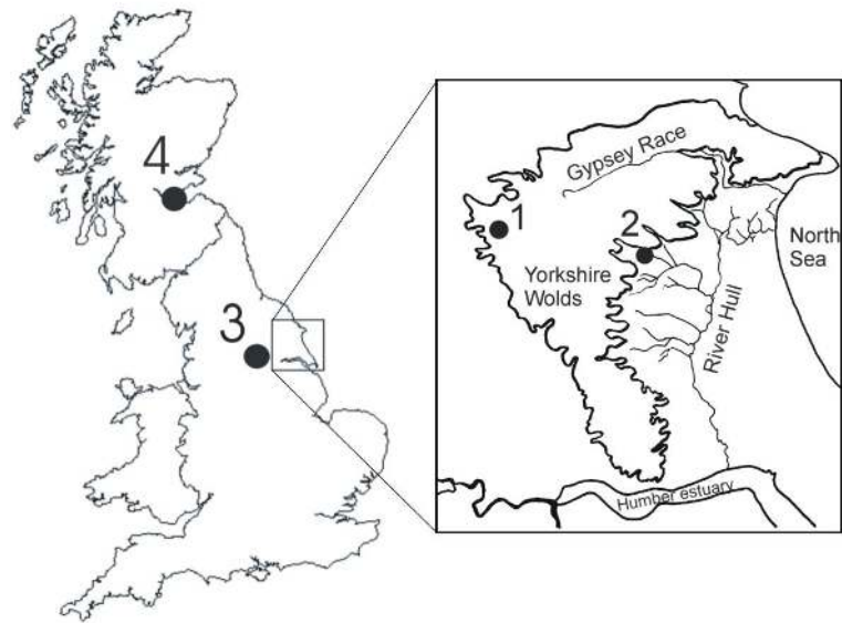
Figure 1. Map showing the East Yorkshire Wolds area (heavy black outline is the 60m contour), with drainage to the east into the River Hull, on lower ground between the chalk Wolds and the North Sea coast. The Humber estuary is to the south of the Wolds and the seasonal watercourse of the Gypsy Race is in the northern high ground. The sites mentioned in the text are marked as: (1) Wetwang and Garton Slacks, and Wetwang Village; (2) Garton Station and Kirkburn; (3) Ferry Fryston; (4) Newbridge.
