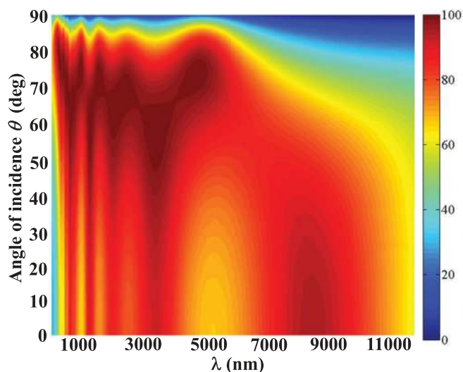
FIG. 2. (Color online) Angular absorption spectra for the structure in Fig. 1(a) with period d = 96 nm and slit width w = 24 nm with \epsilon_S = 1 . The grating and taper lengths are l = 200 nm and l_{tap} = 980 nm, respectively. Broadband omnidirectional absorption is obtained at optical and IR frequencies.
