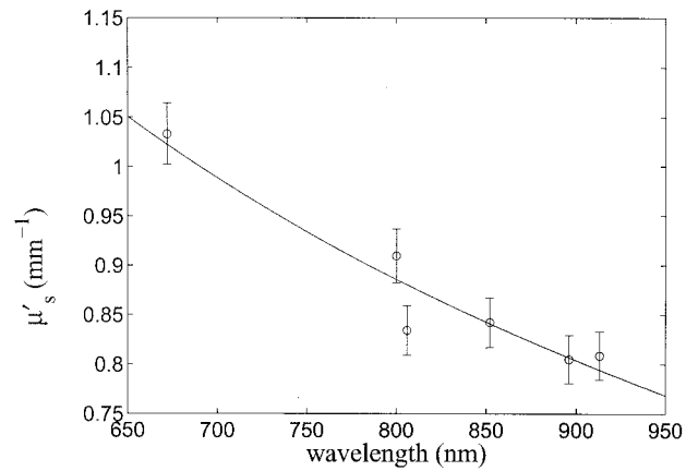
Fig. 4. Determination of the broadband \mu'_s spectrum for the dye-Intralipid phantom. Open circles, discrete \mu'_s values measured by the FD technique; solid curve, best power-law fit to Eq. (4). Fitting parameters are A = 2200 and B = -0.82 . Error bars on \mu'_s are 3%. 7
